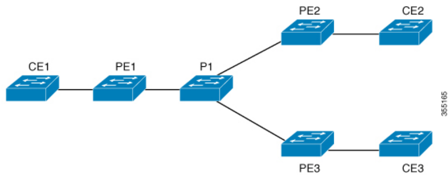
Figure 24: VPLS Topology
