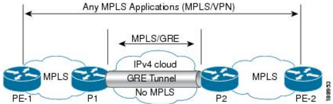
Figure 21: P-to-P Tunneling
