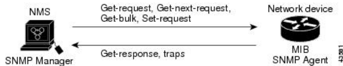
Figure 2: SNMP Network
