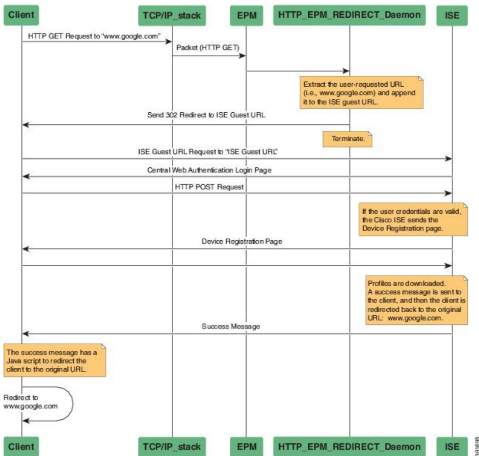
Figure 36: Original URL Redirection Packet Flow
