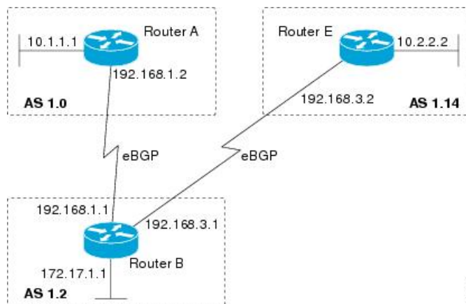
Figure 14: BGP Peers Using 4-Byte Autonomous System Numbers in Asdot Format
