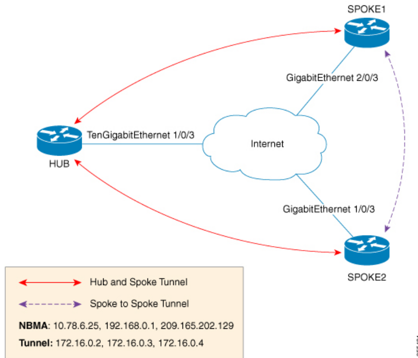
Figure 20: Sample mGRE Configuration at Hub and Spokes
