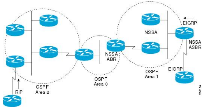
Figure 5: OSPF NSSA
