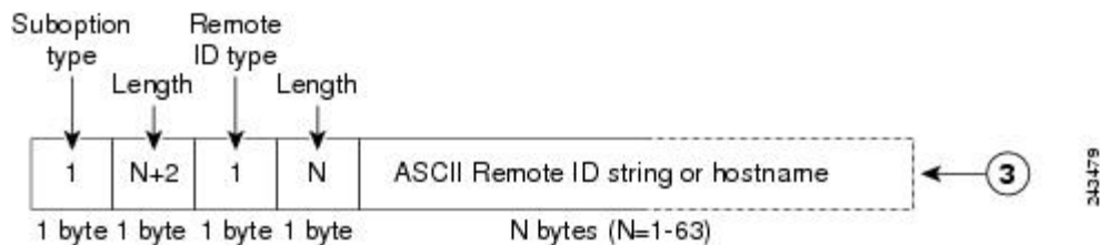
Figure 24: Suboption Packet Formats, Remote ID Specified
