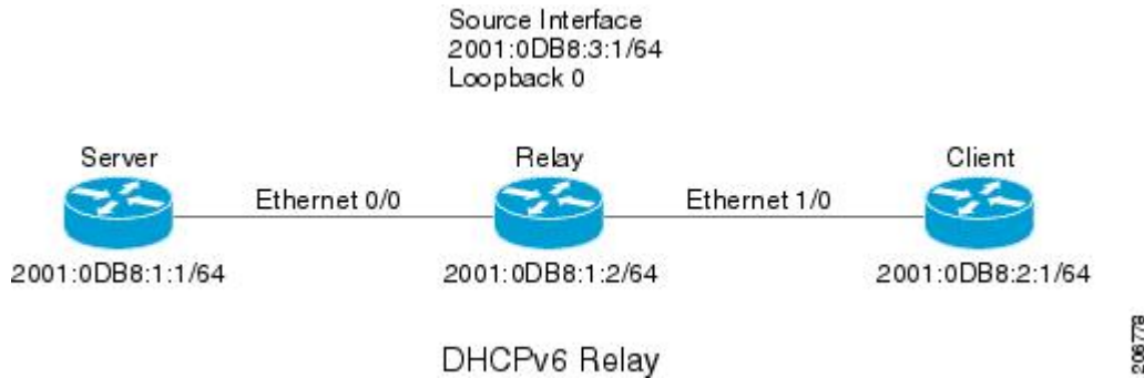
Figure 25: DHCPv6 Relay Source Configuration—Simple Network
