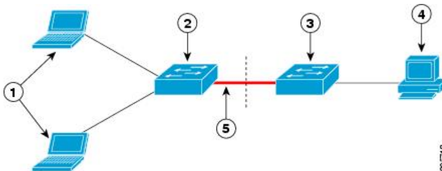
Figure 31: Authenticator and Supplicant Switch using CISP
