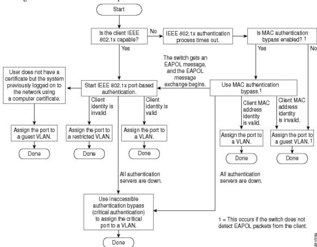
Figure 34: Authentication Flowchart
