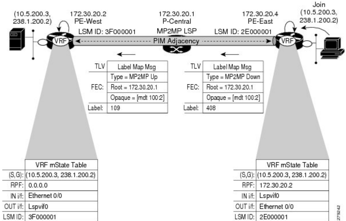
Figure 42: PIM Signaling over LSP
