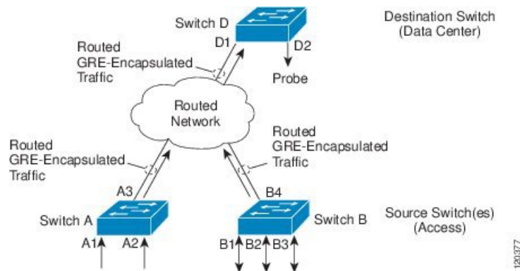
Figure 9: ERSPAN Configuration
