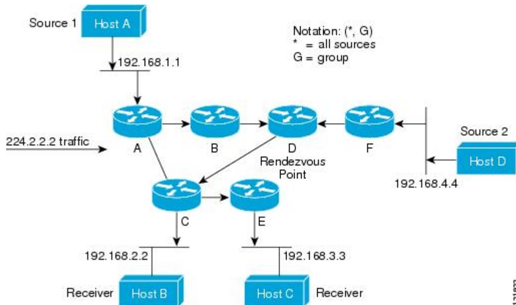
Figure 14: Shared Tree
