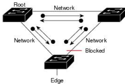
Figure 27: Network with STP Topology Running Bridge Assurance
