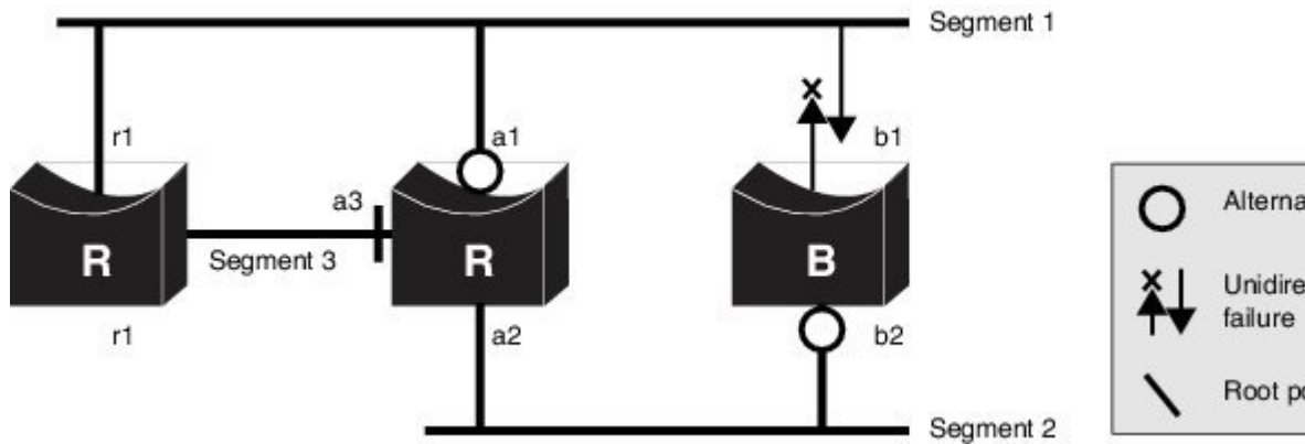
Figure 16: Bridging Loops on Shared Segments
