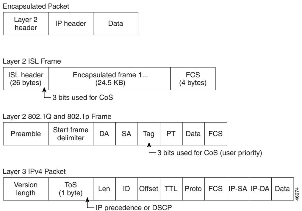
Figure 32-1 QoS Classification Layers in Frames and Packets
