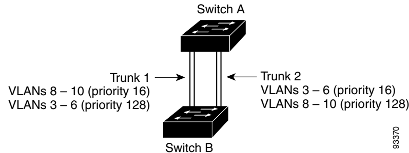
Figure 13-2 Load Sharing by Using STP Port Priorities
