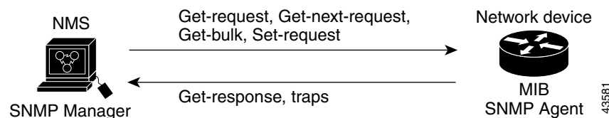
Figure 29-1 SNMP Network
