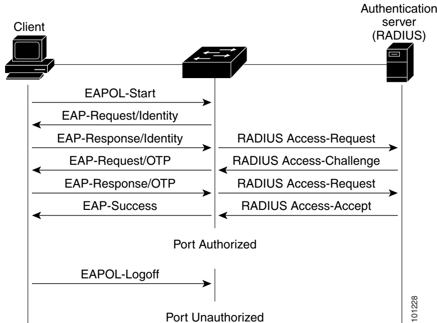
Figure 12-3 Message Exchange
