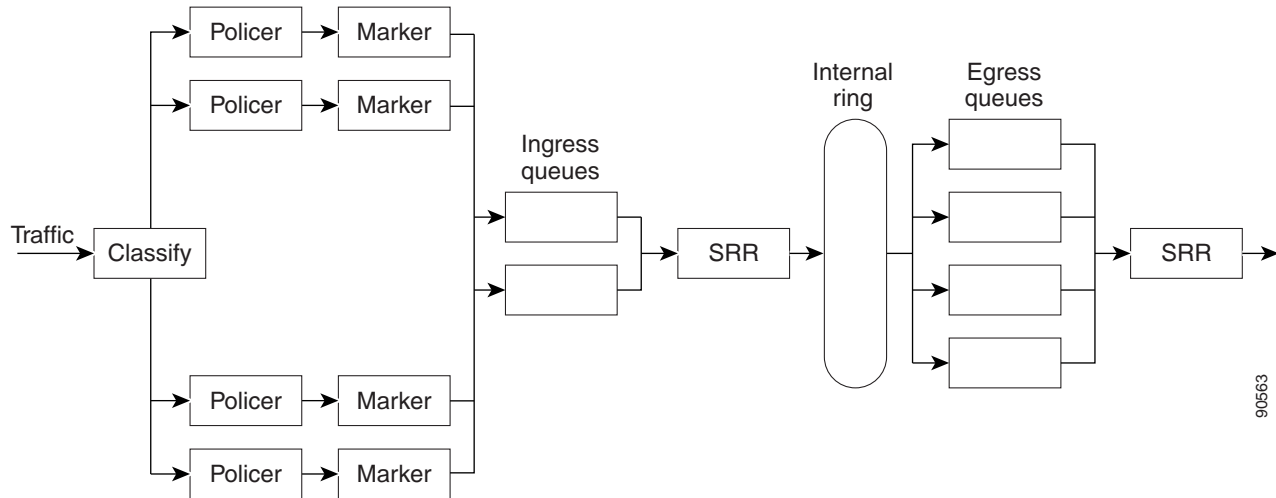
Figure 35-6 Ingress and Egress Queue Location
