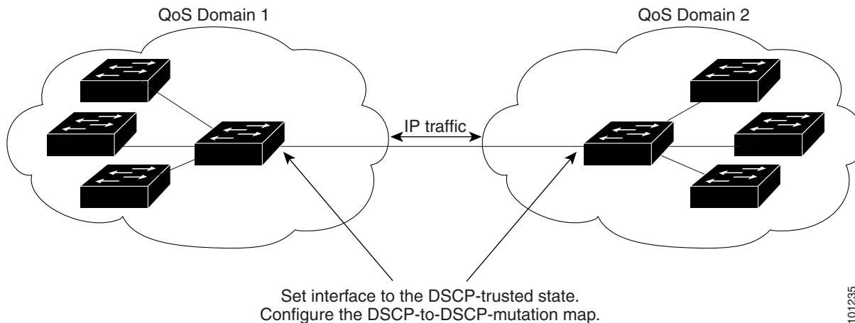
Figure 39-12 DSCP-Trusted State on a Port Bordering Another QoS Domain
