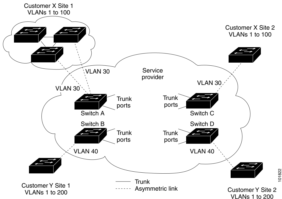
Figure 20-4 Layer 2 Protocol Tunneling
