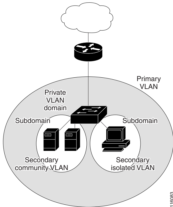
Figure 19-1 Private-VLAN Domain
