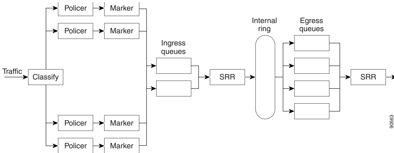
Figure 39-6 Ingress and Egress Queue Location
