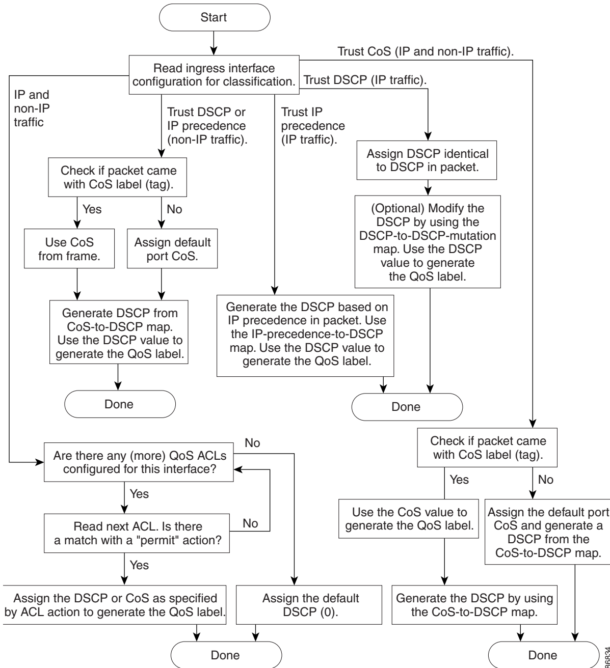
Figure 39-3 Classification Flowchart
