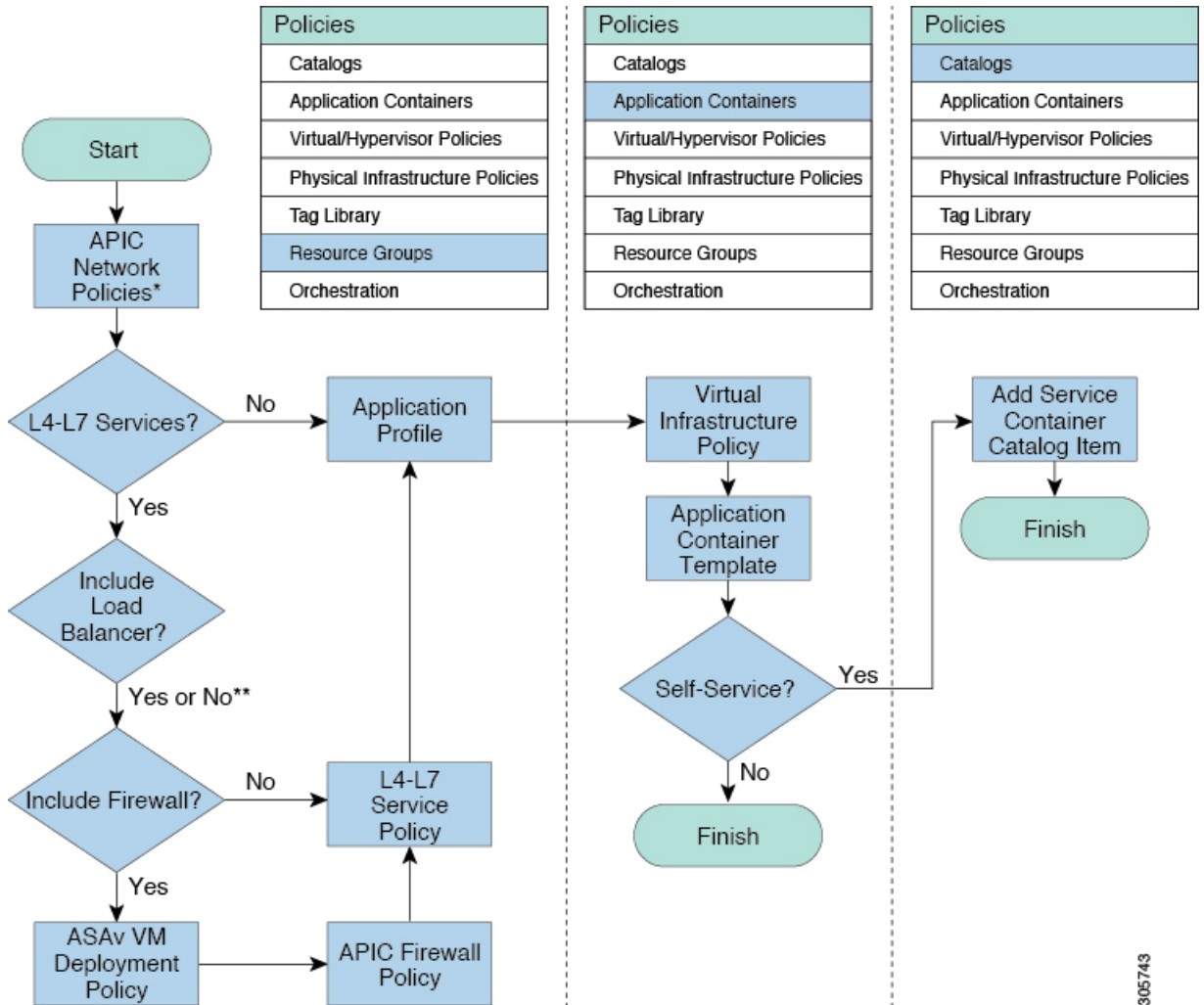
Figure 3: Process for Creating an APIC Application Container
