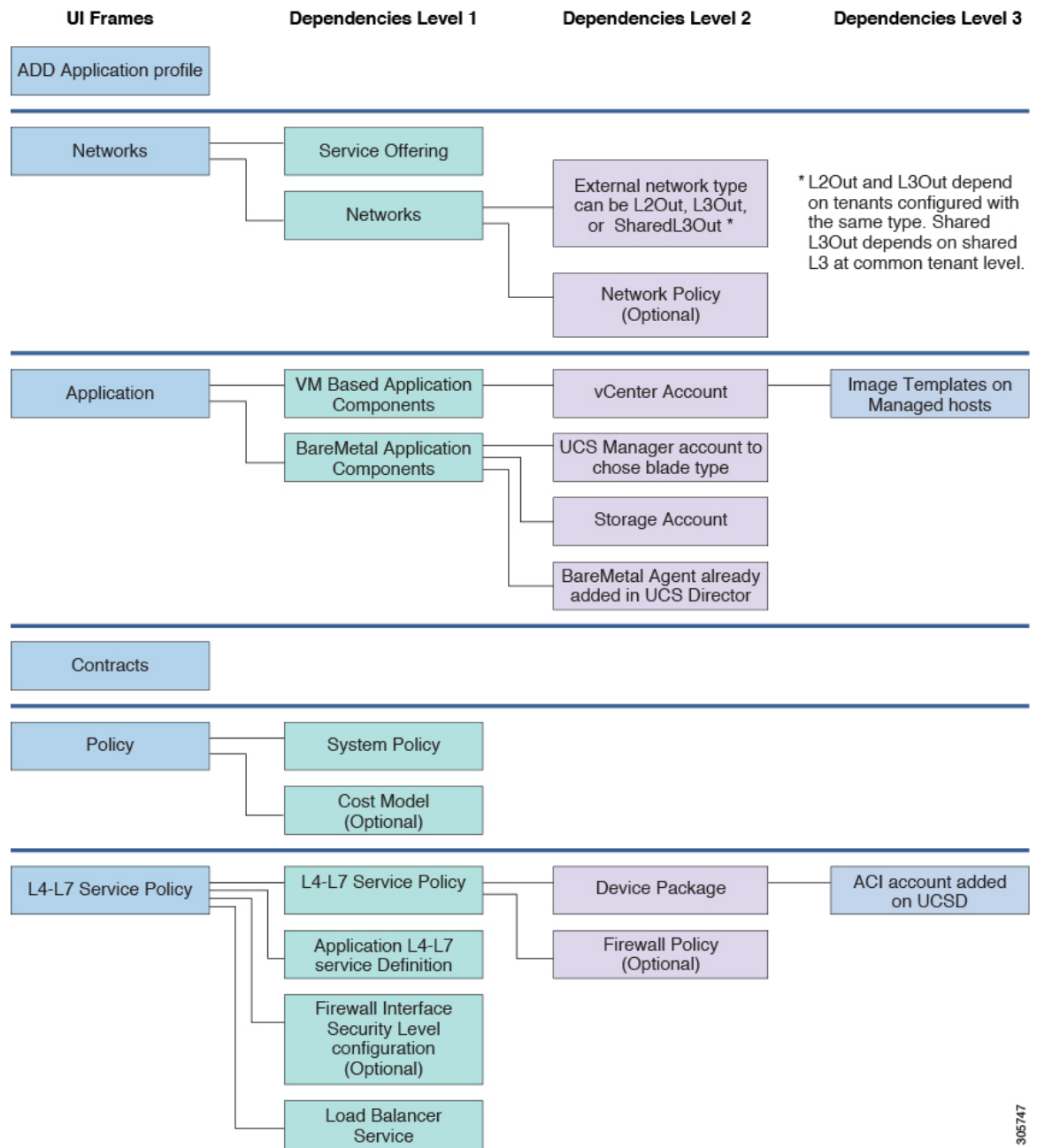
Figure 4: Application Profile — Dependencies
