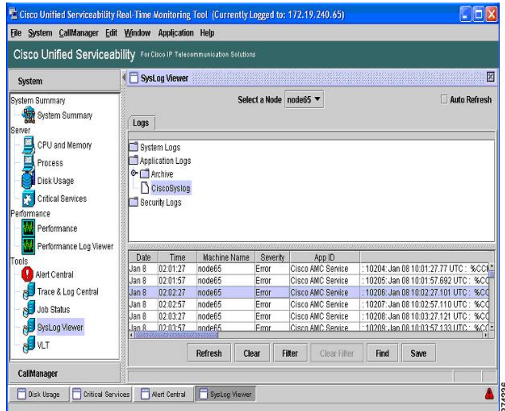
Figure 11: Syslog Viewer
