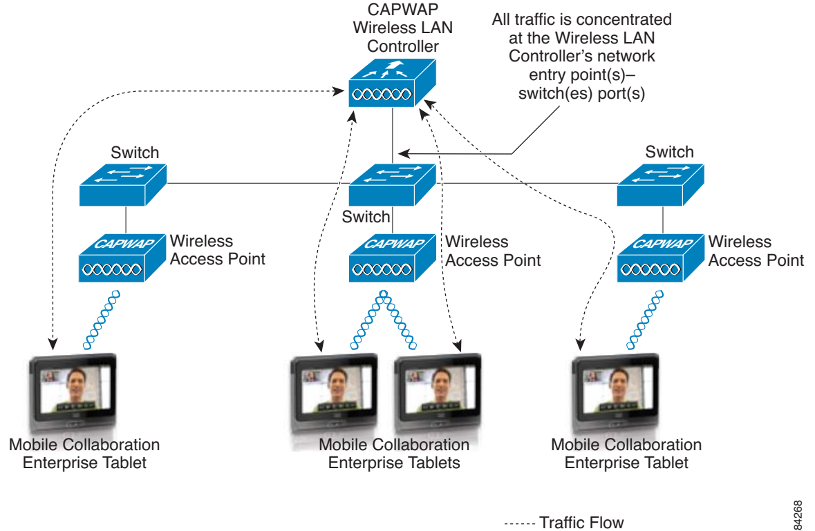
Figure 3-22 Traffic Concentrated at the Wireless LAN Controller Network Entry Point
