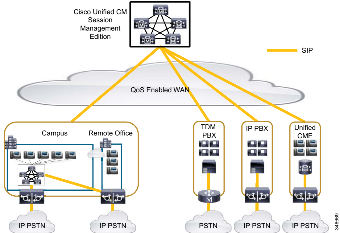
Figure 6-31 Distributed SIP Trunk Model
