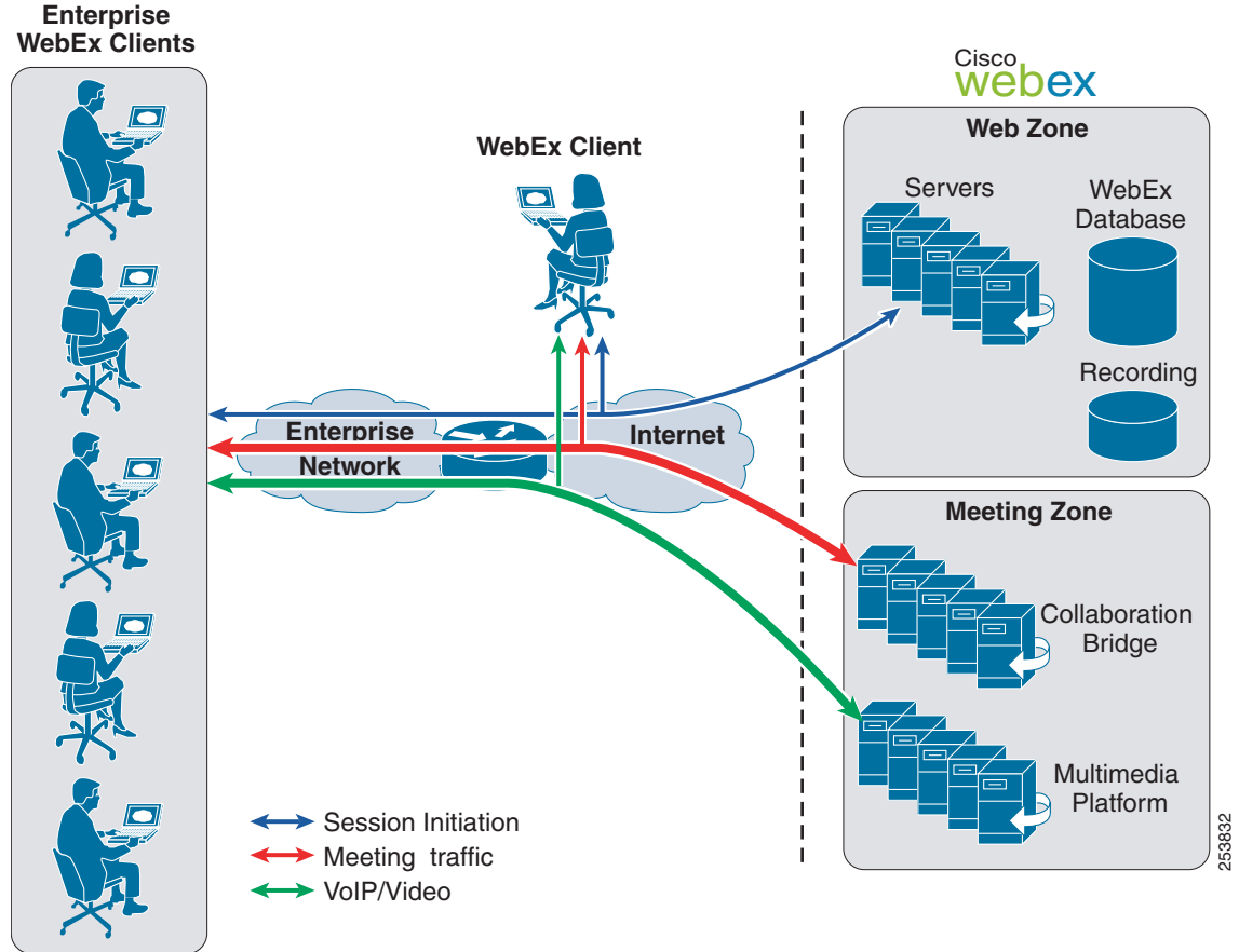
Figure 22-3 WebEx Deployment
