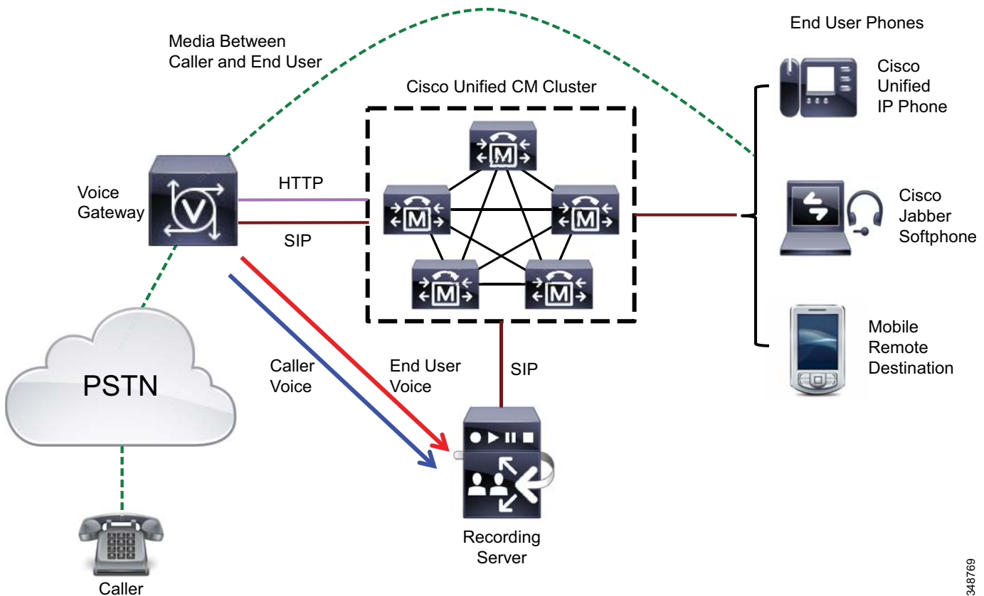
Figure 25-3 Basic Setup for Cisco Unified CM Network-Based Recording
