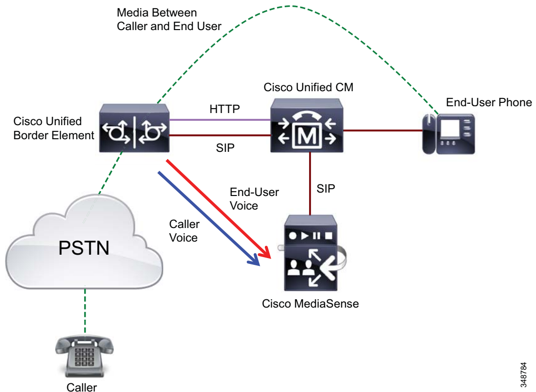
Figure 25-6 Integration of Cisco MediaSense and Unified CM Network-Based Recording
