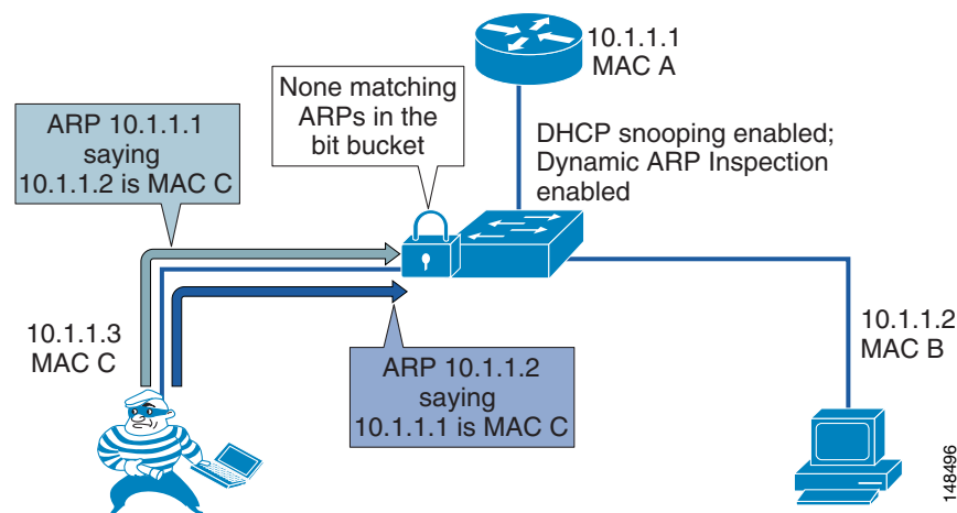
Figure 4-7 Using DHCP Snooping and DAI to Block ARP Attacks
