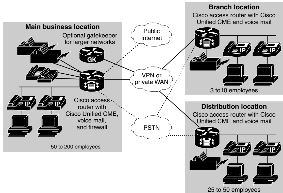
Figure 3-3 Multisite Distributed Cisco Unified CME Network Topology
