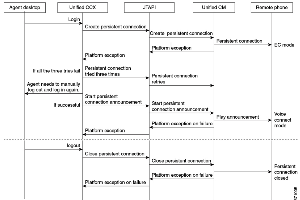
Figure 14: Signaling Flow
