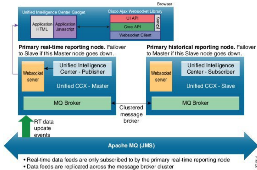
Figure 18: System Architecture - Cisco Unified Contact Center Express
