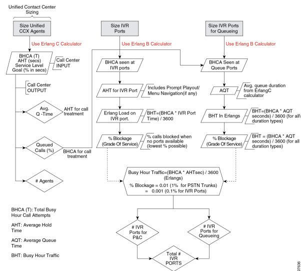
Figure 16: Call Center Sizing - Voice Only
