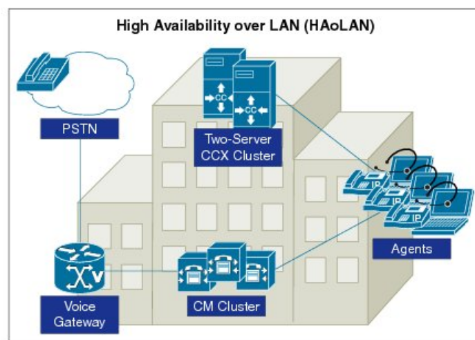
Figure 20: Unified CCX High Availability over LAN Deployment
