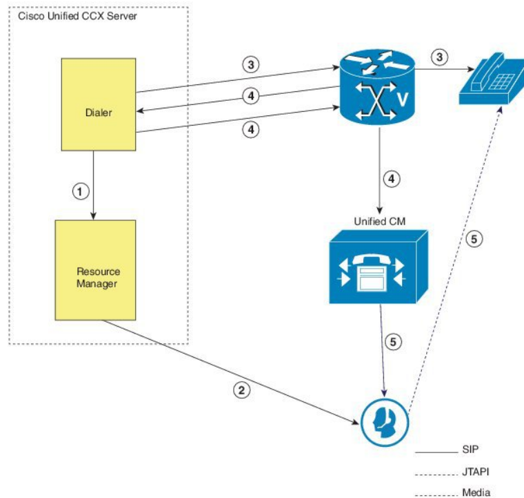
Figure 6: Call Flow for Agent Mode
