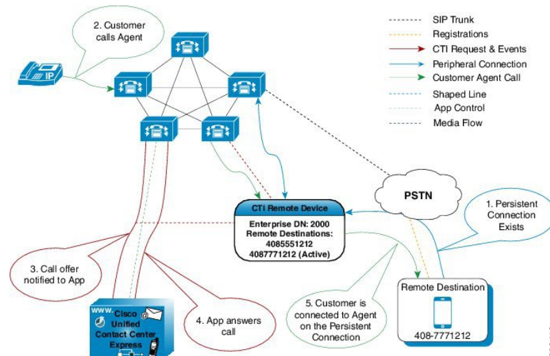
Figure 13: Persistent Connection Incoming Call
