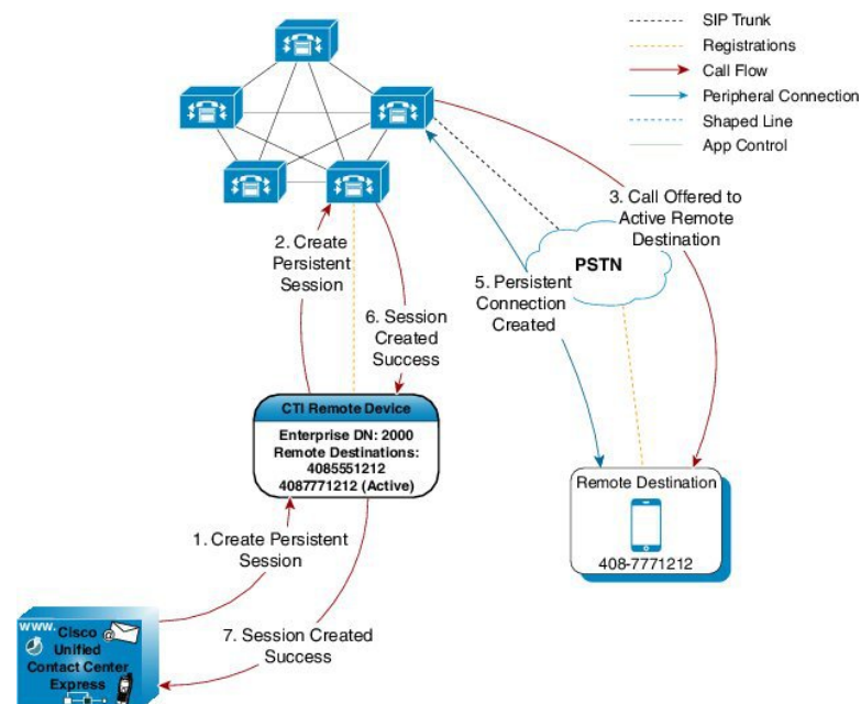
Figure 12: Persistent Connection Call Flow
