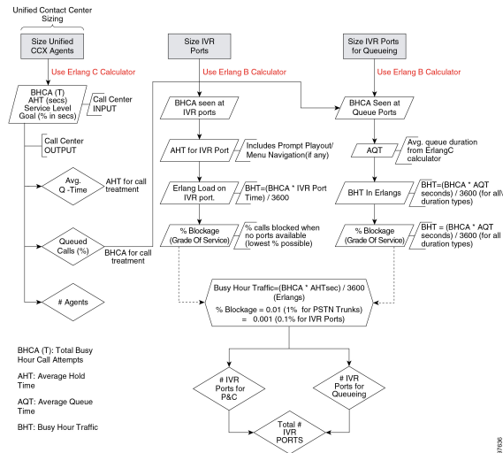
Figure 17: Call Center Port Types
