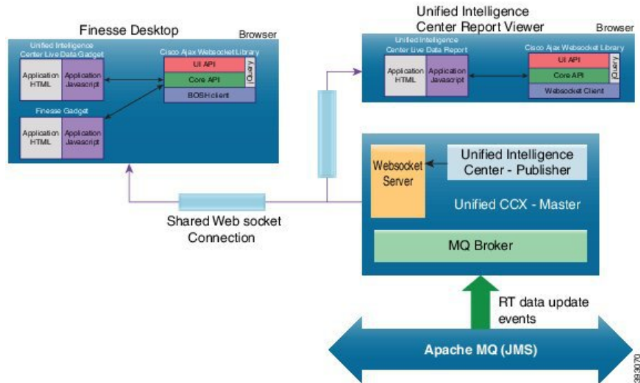
Figure 19: Cisco Unified Contact Center Express - Live Data Gadgets
