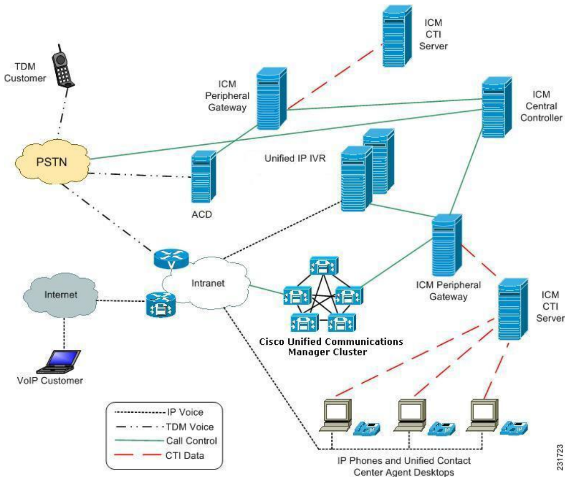
Figure 3: A Unified Deployment Model within Unified CCE
