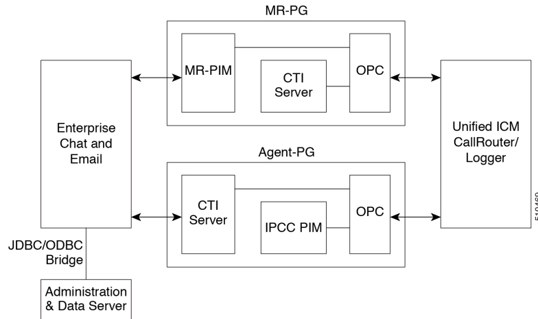
Figure 35: Interfacing with Enterprise Chat and Email
