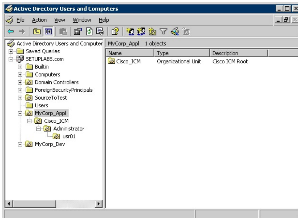
Figure 28: SETUPLABS Domain
