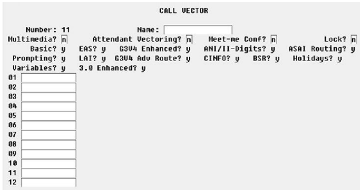
Figure 8: Vector
