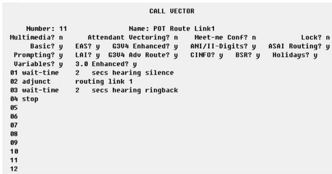
Figure 9: Call Vector
