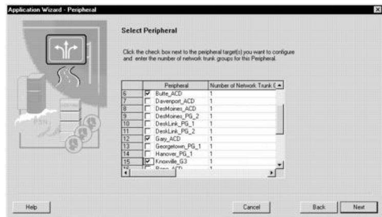
Figure 26: Application Wizard—Peripheral
