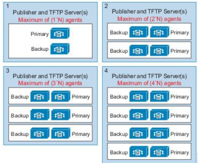
Figure 97: Redundancy Configuration Options
