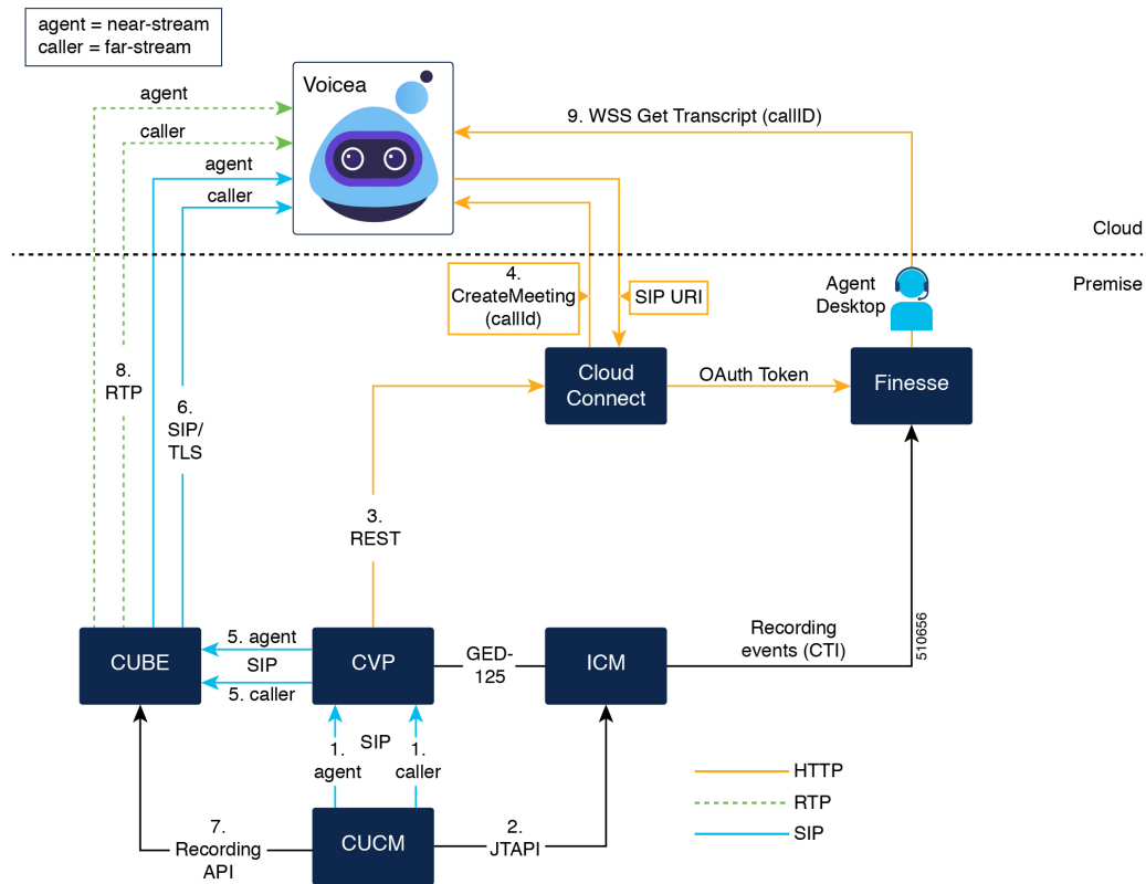
Figure 74: Call Transcript Call Flow
