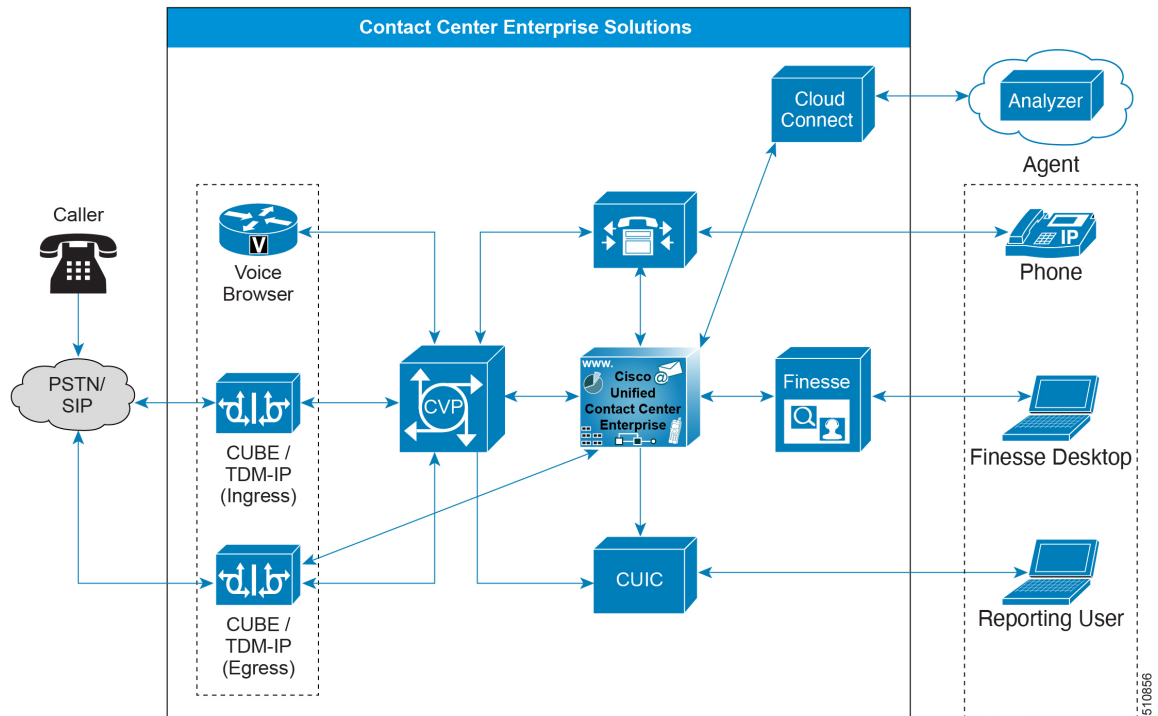
Figure 121: Customer Journey Analyzer Call Flow
