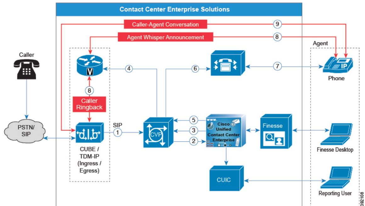
Figure 122: Whisper Announcement Call Flow
