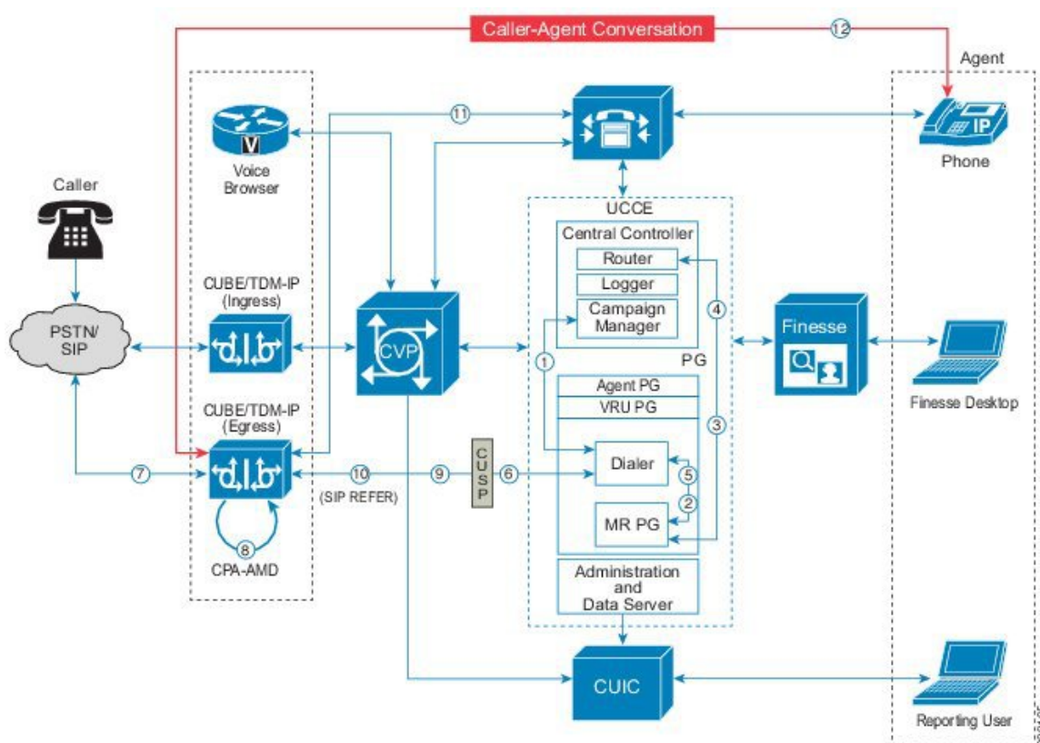
Figure 104: SIP Dialer Agent Campaign Call Flow
