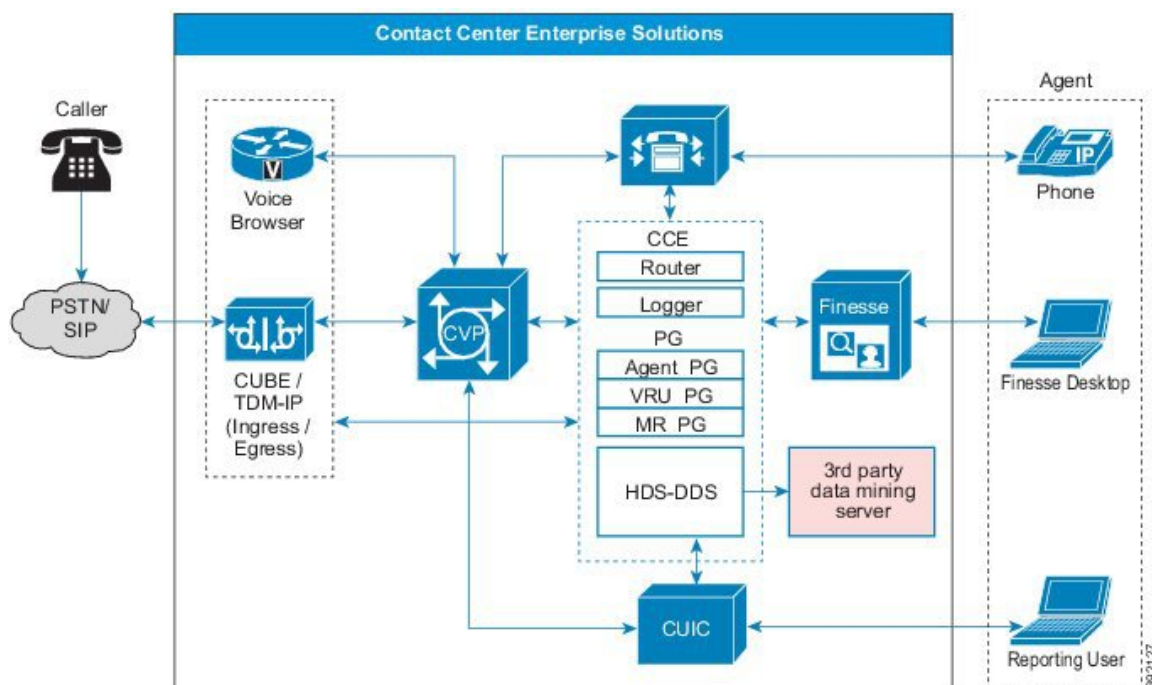
Figure 20: Historical Data Server and Detail Data Server (HDS-DDS)
