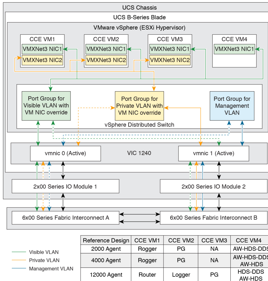
Figure 80: Network Requirements for Cisco UCS B-Series Servers
