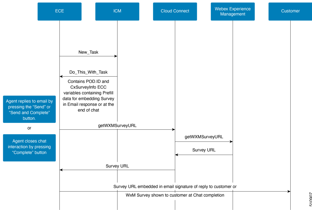
Figure 120: Email/Chat Survey Call Flow
