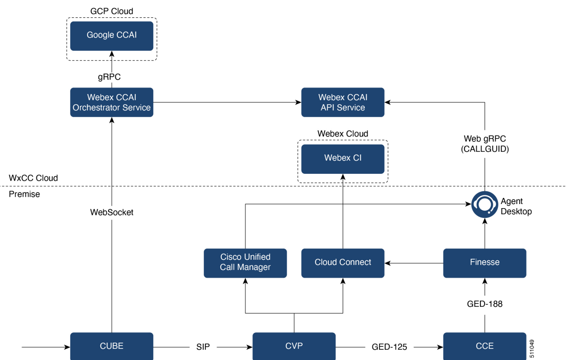
Figure 112: Contact Center AI Services Architecture
