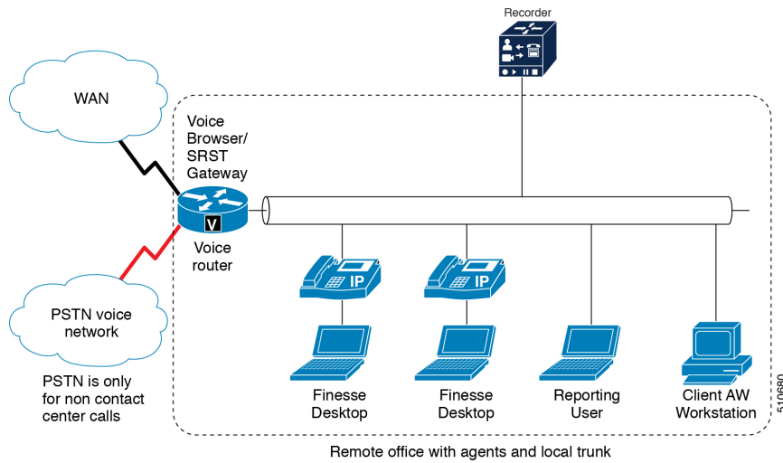
Figure 50: Remote Office with Agents and Voice Gateway—Physical View
