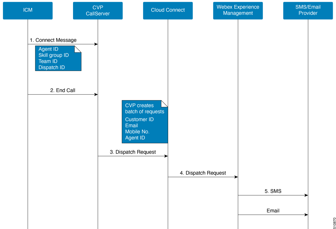
Figure 118: Email/SMS Survey Call Flow
