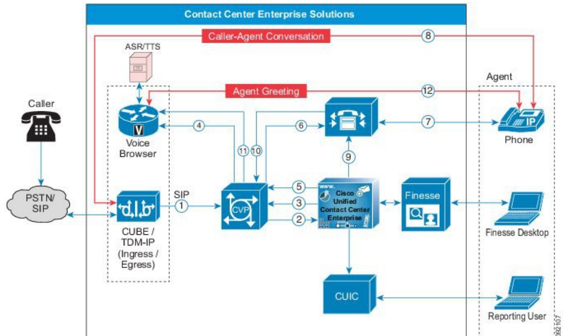
Figure 100: Agent Greeting Call Flow
