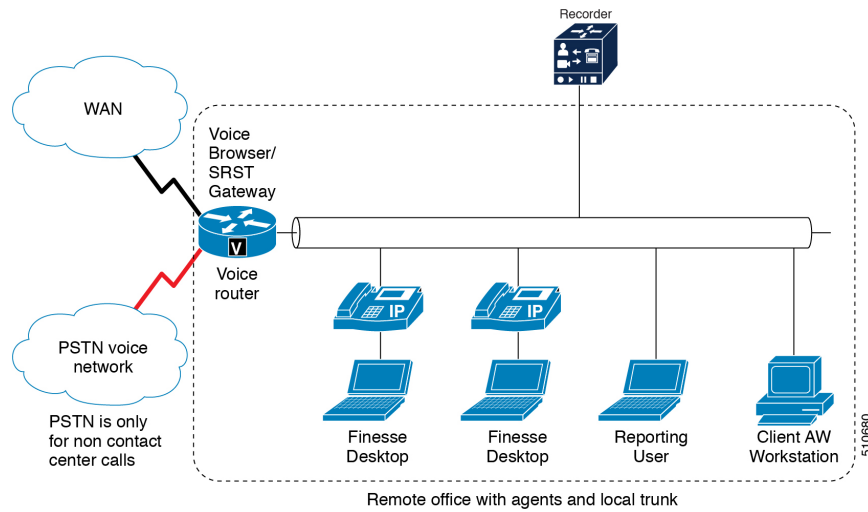
Figure 41: Remote Office with Agents and Voice Gateway—Physical View
