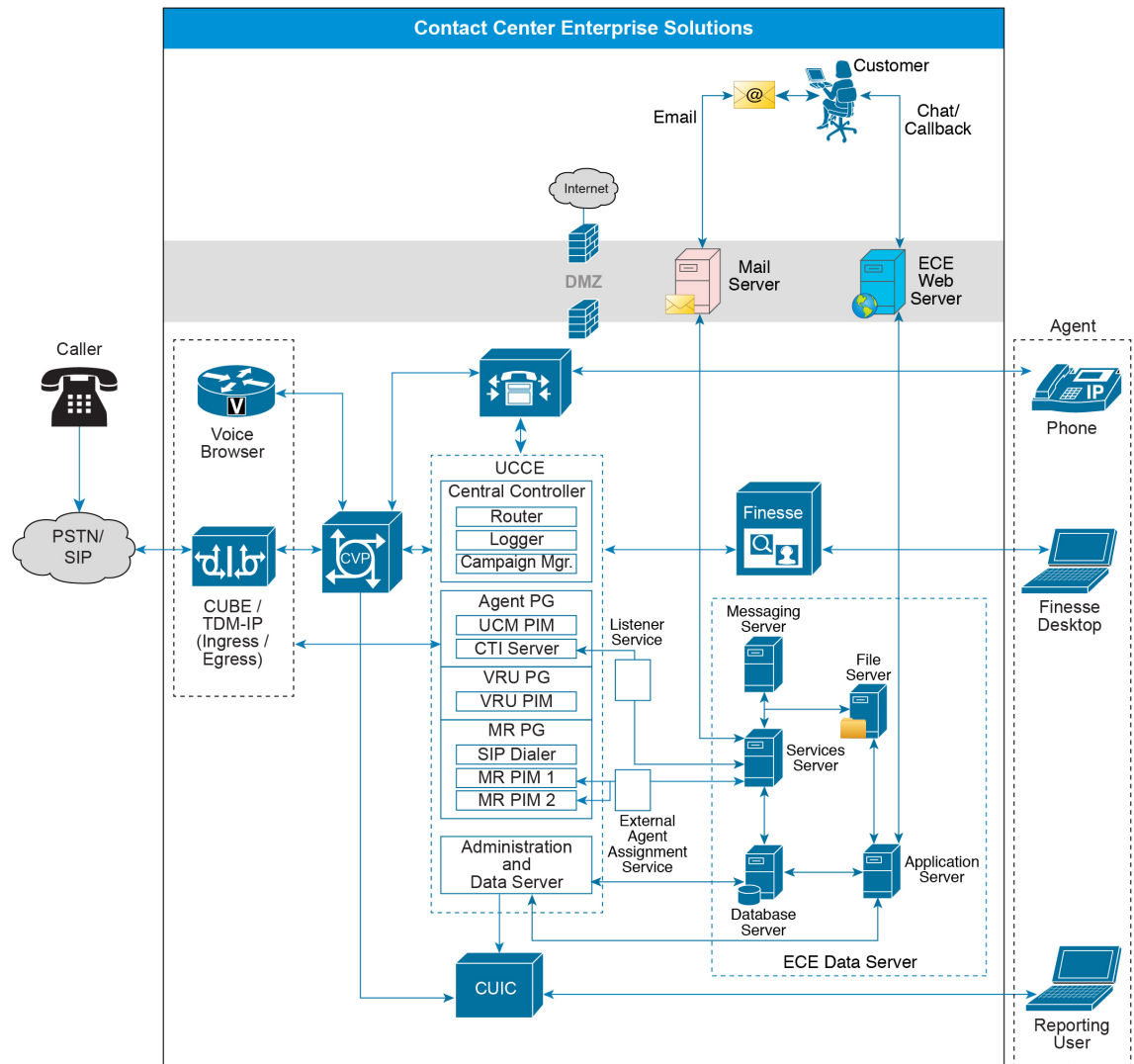
Figure 69: Enterprise Chat and Email Design Considerations
