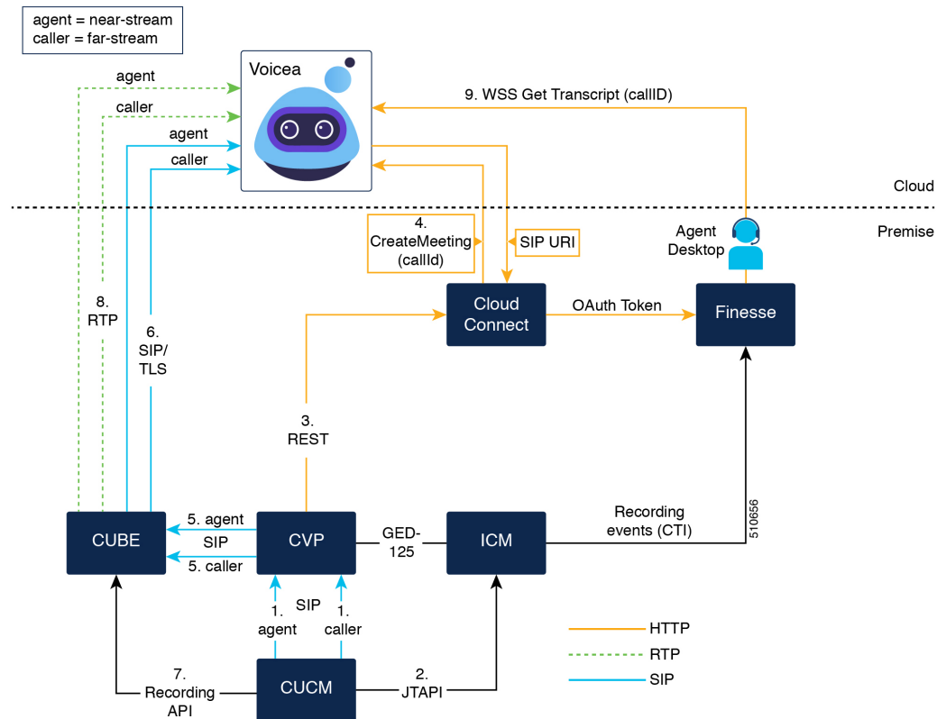
Figure 72: Call Transcript Call Flow
