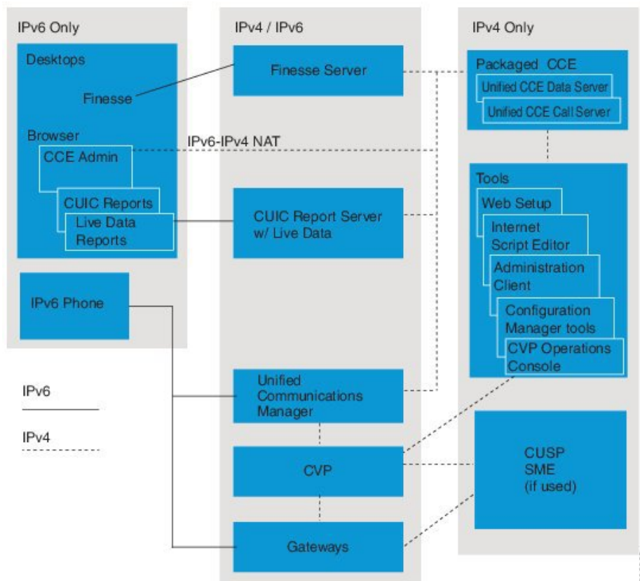
Figure 118: Packaged CCE Deployment with Only IPv6 Agents
