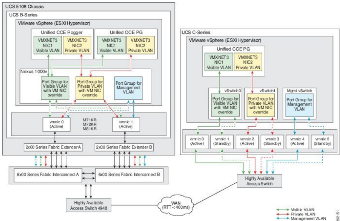
Figure 67: UCS Network Reference Design for Global Deployment
