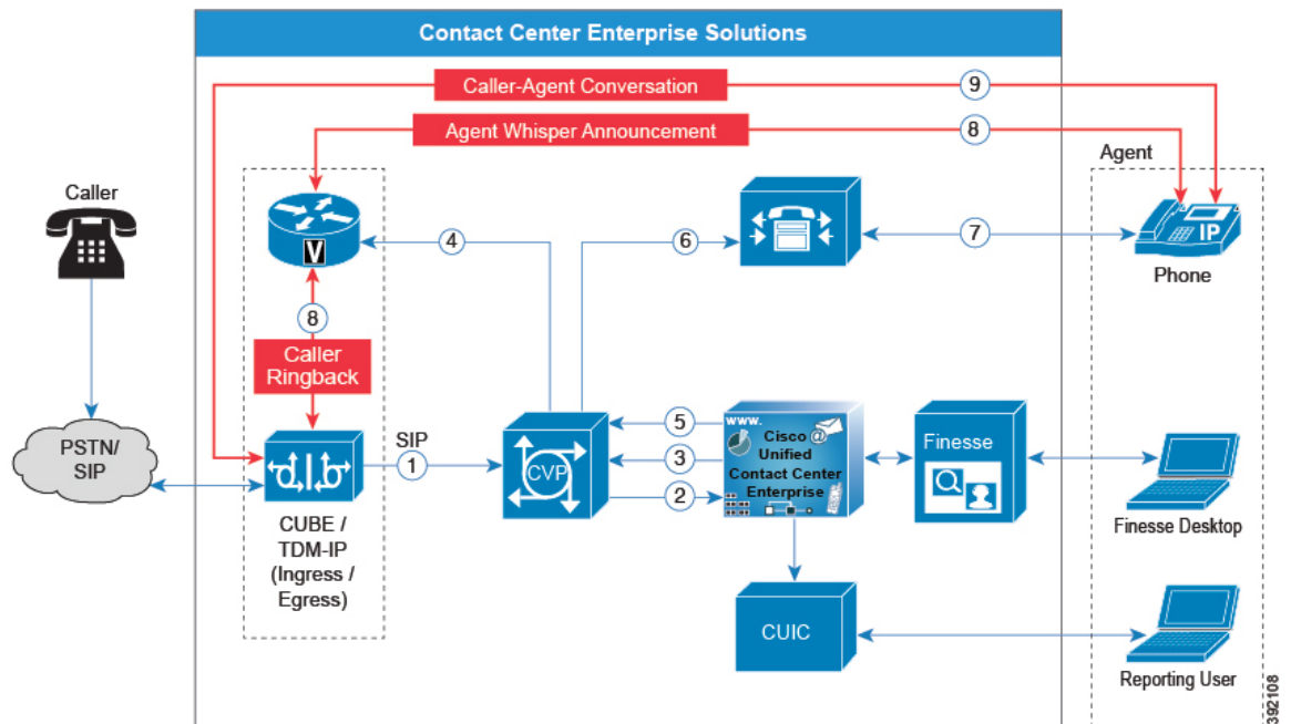
Figure 116: Whisper Announcement Call Flow
