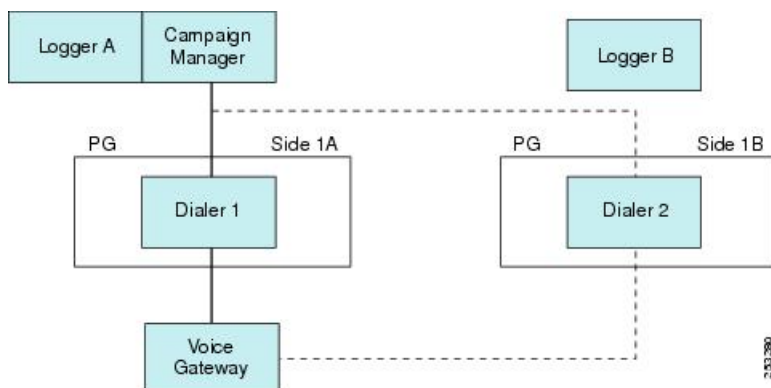
Figure 106: Single Gateway Deployment for SIP Dialer
