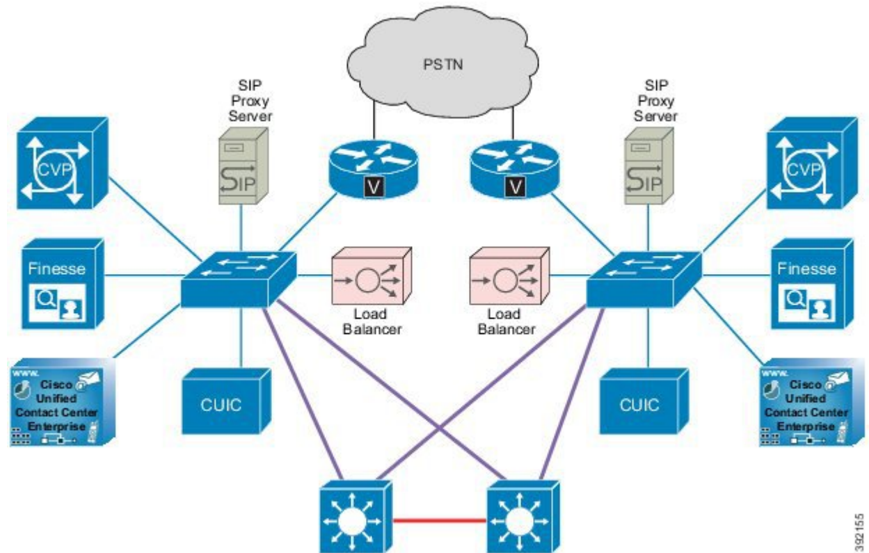
Figure 84: Redundant Unified CVP System
