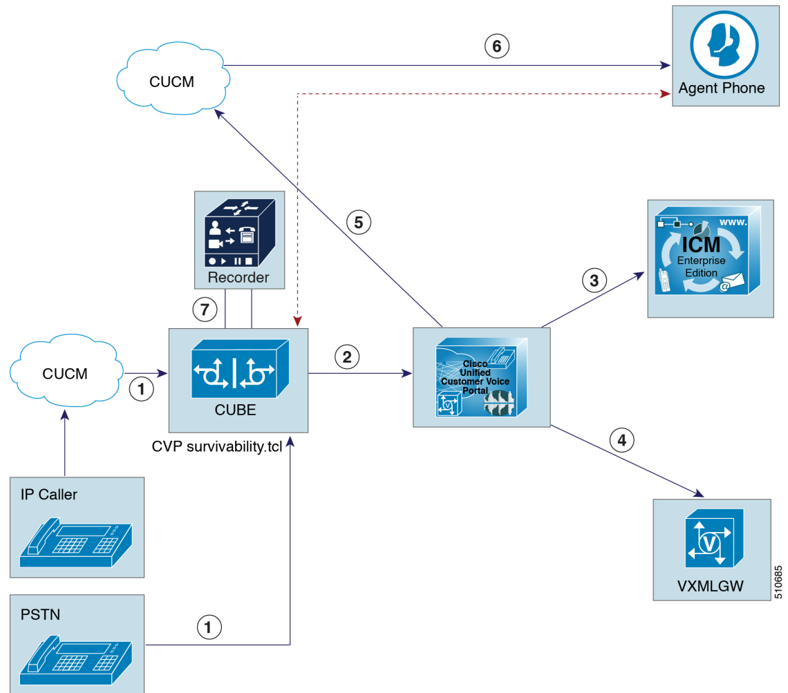
Figure 74: Network-Based Recording Call Flow
