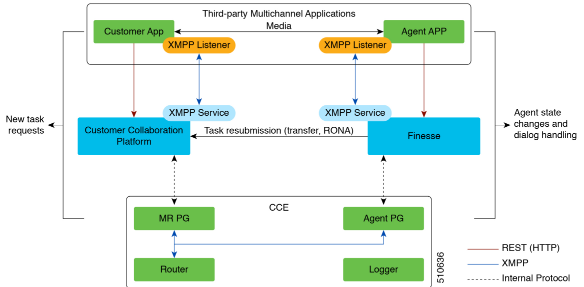
Figure 68: Task Routing for Third-party Multichannel Applications Solution Components
