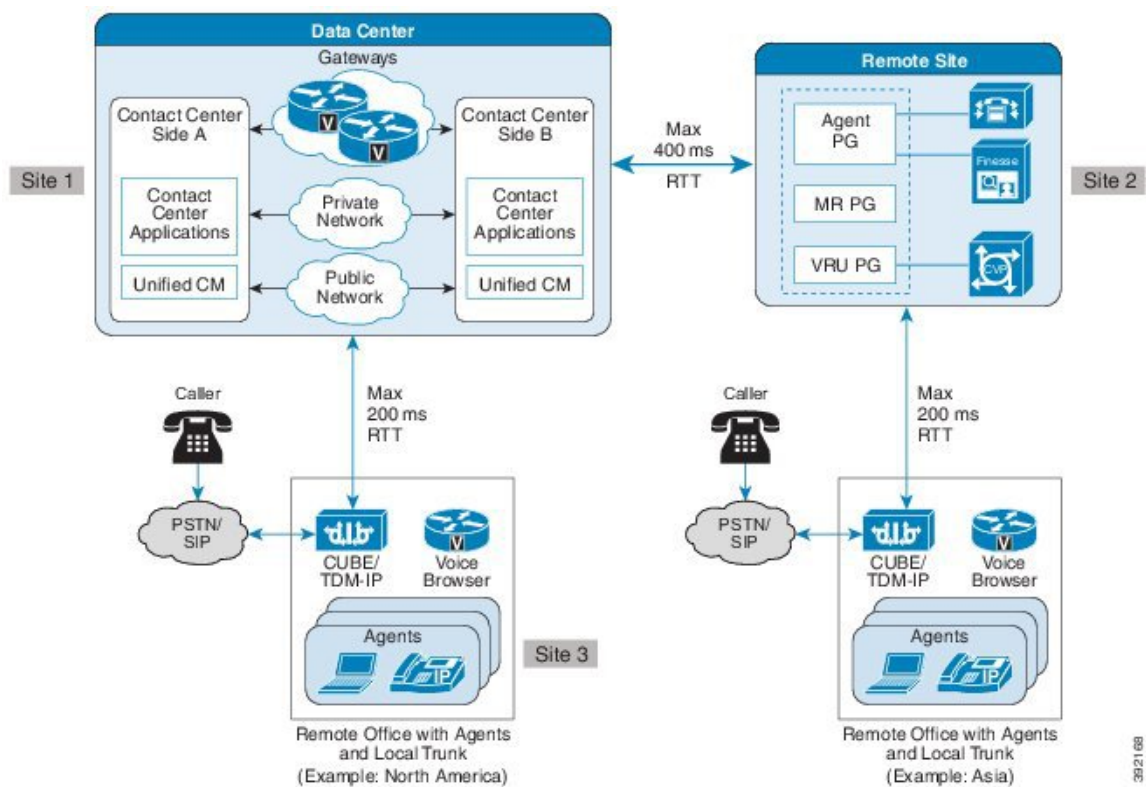
Figure 109: Distributed Outbound SIP Dialer Deployment for an Agent-Based Campaign
