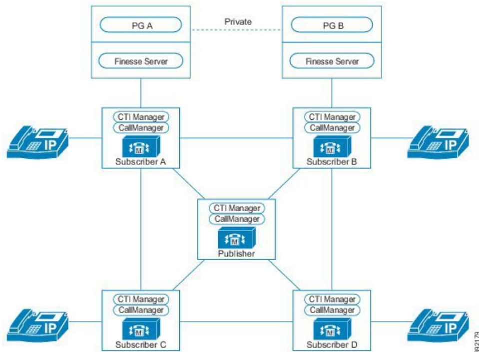
Figure 61: Single Agent PG Pair for Entire Unified CM Cluster
