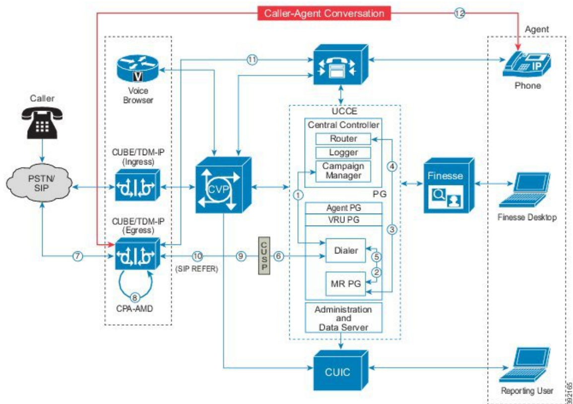
Figure 104: SIP Dialer Agent Campaign Call Flow
