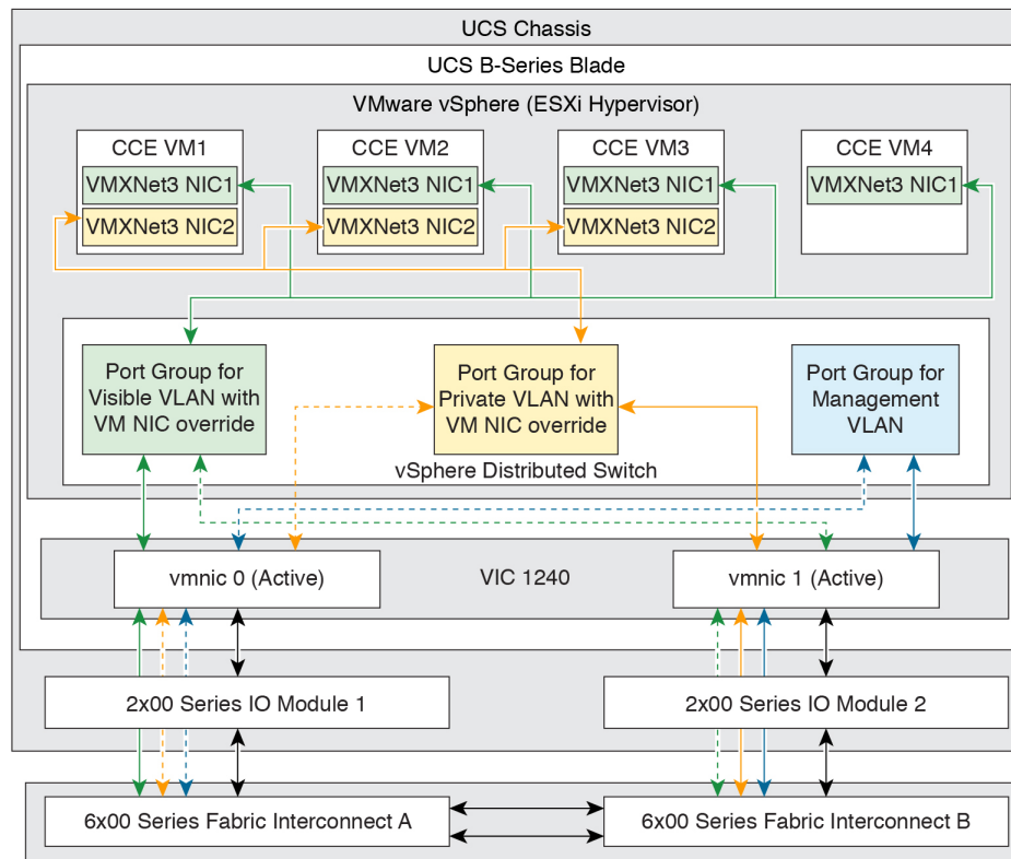
Figure 78: Network Requirements for Cisco UCS B-Series Servers
