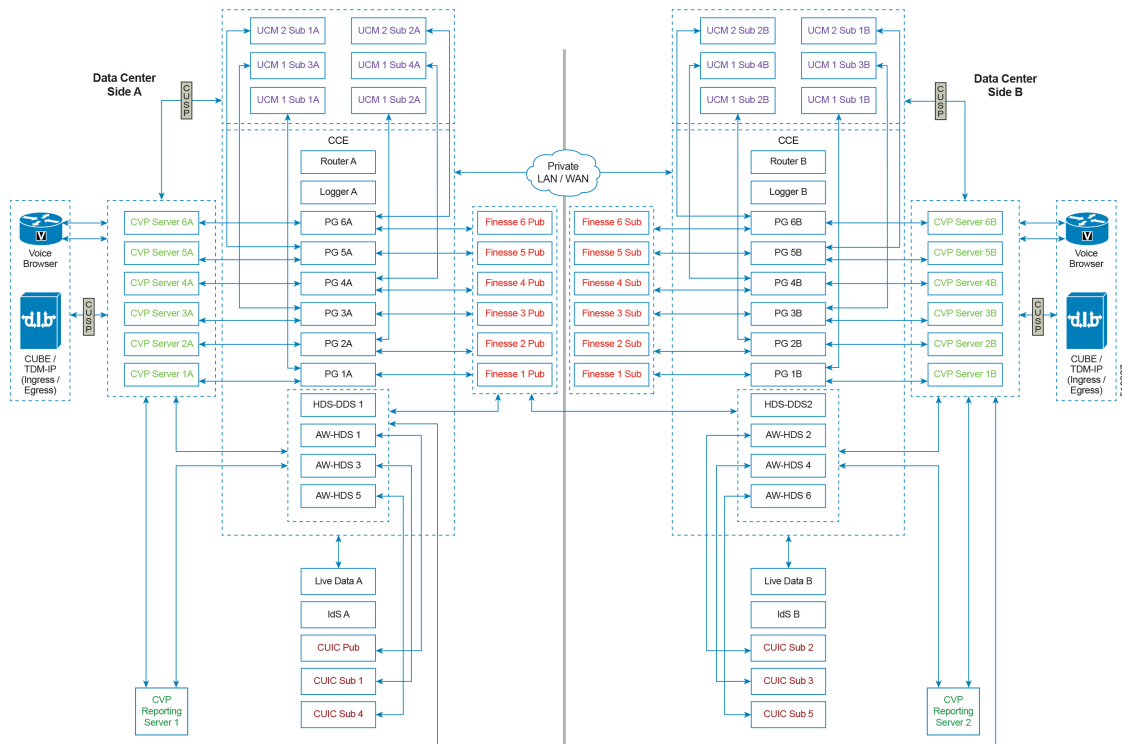
Figure 54: Detailed 12000 Agent Reference Design
