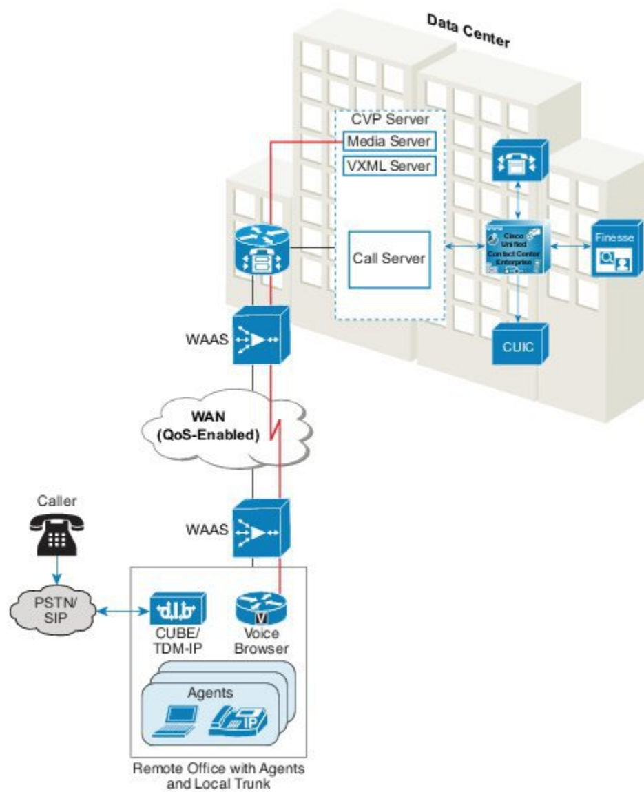
Figure 55: Distributed Deployment Over WAN
