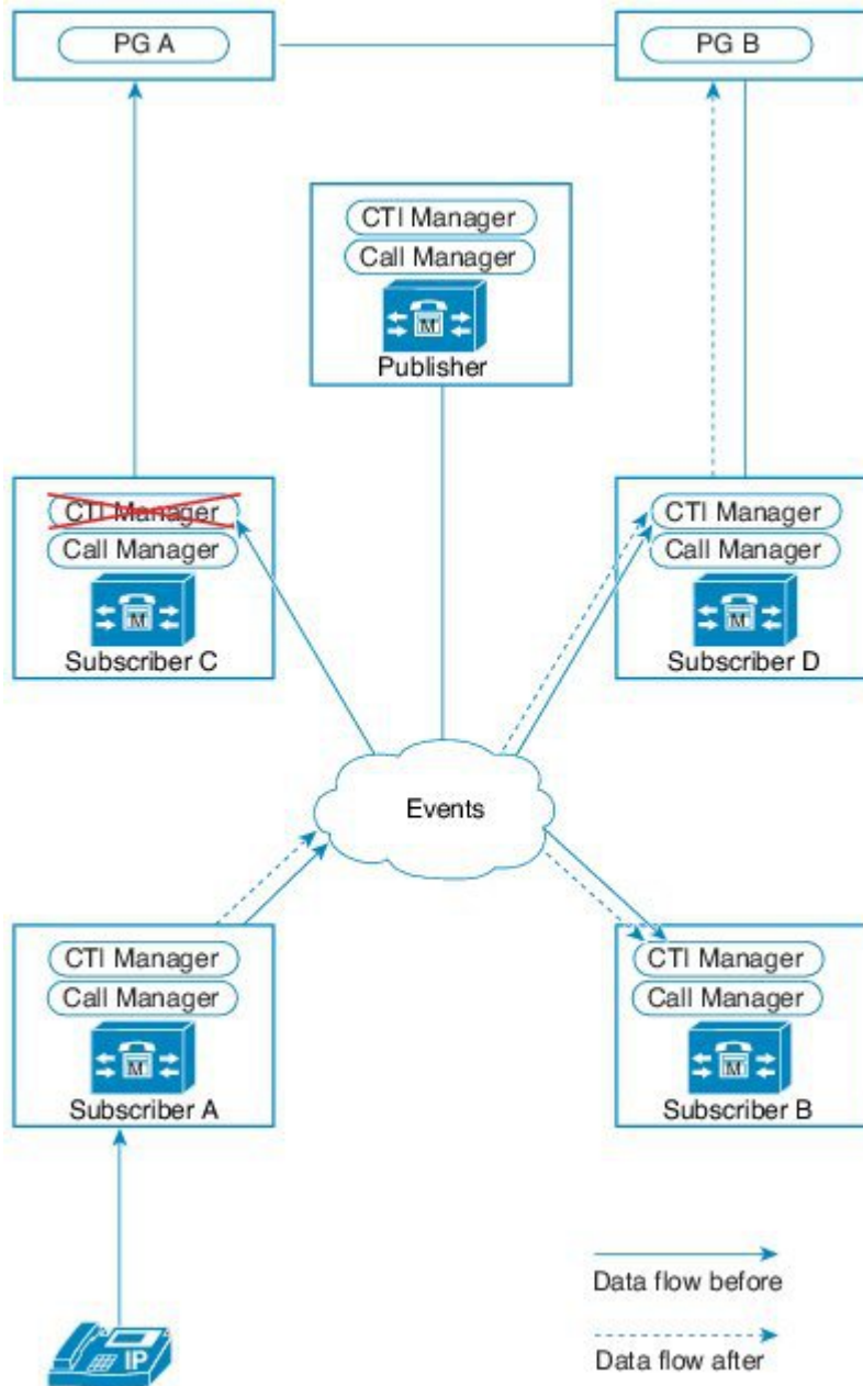
Figure 85: CTI Manager with Agent PG Connection Fails
