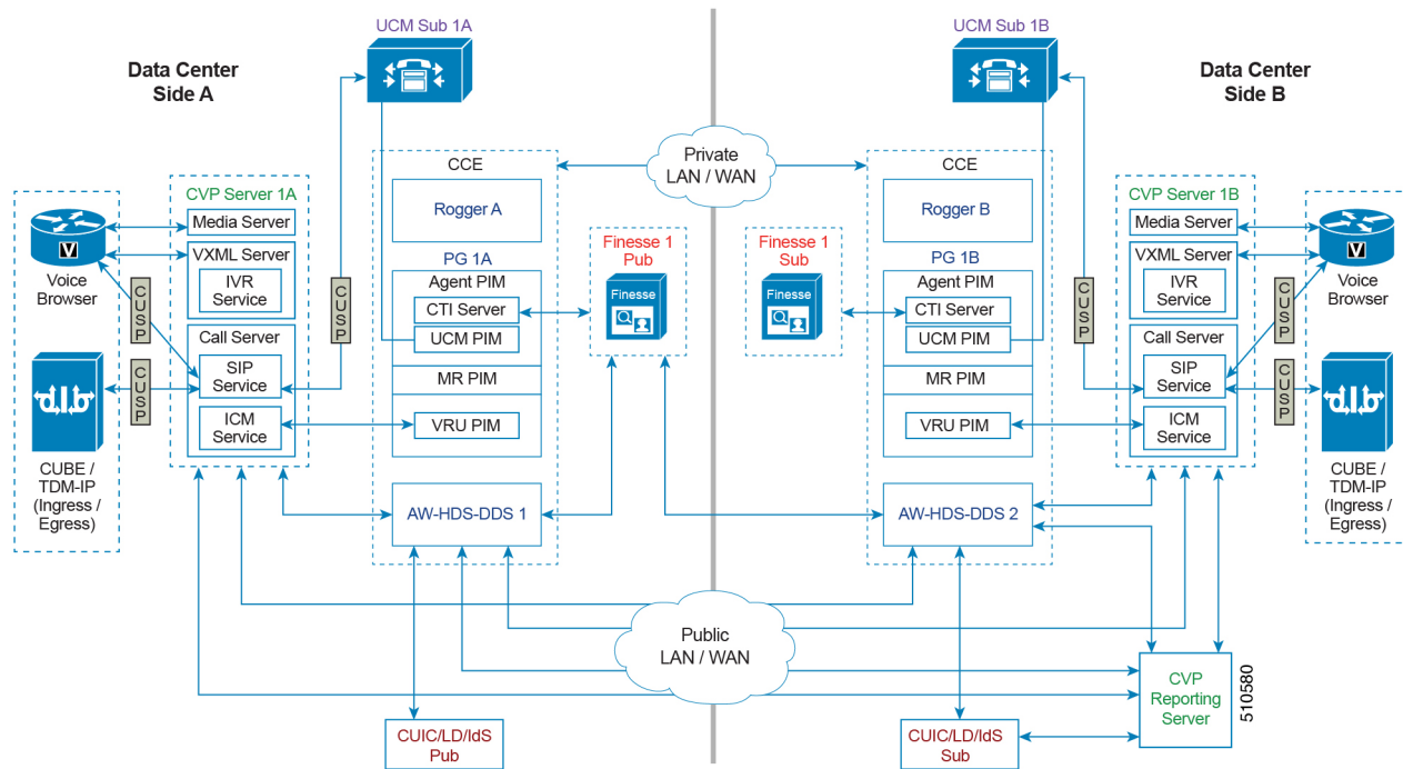
Figure 52: Detailed 2000 Agent Reference Design
