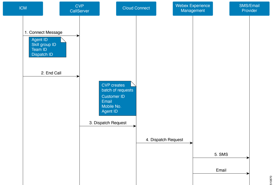
Figure 115: Email/SMS Survey Call Flow
