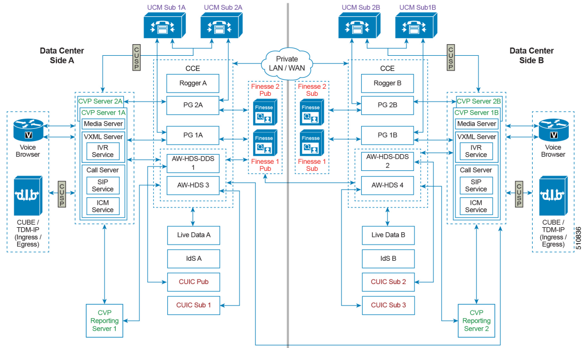
Figure 53: Detailed 4000 Agent Reference Design
