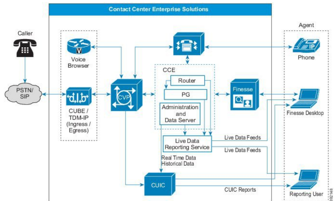
Figure 62: Unified Intelligence Center Deployment
