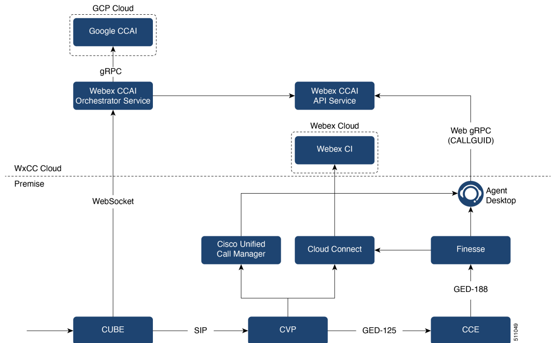
Figure 100: Contact Center AI Services Architecture
