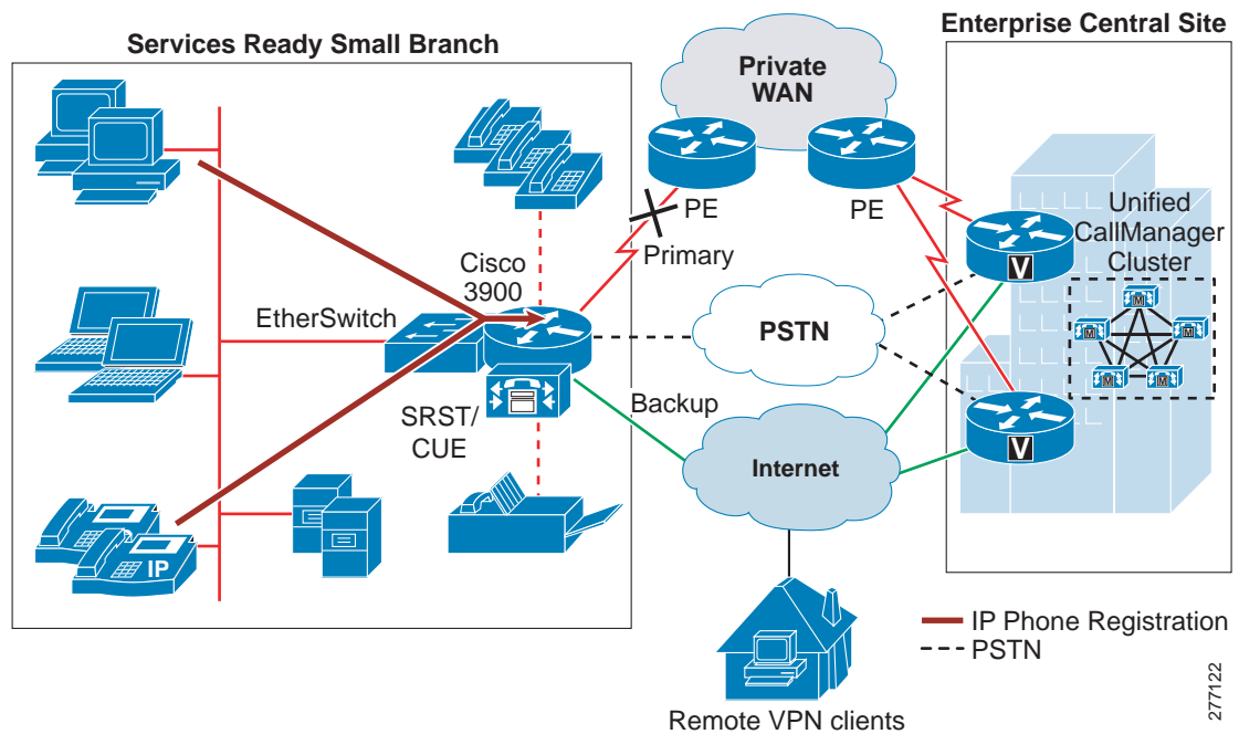
Figure 49 Cisco Unified SRST Mode for Centralized Call Control Model
