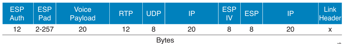
Figure 47 RTP Packet for G.729a Codes with GETVPN Encapsulation
