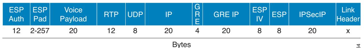
Figure 46 RTP Packet for G.729a Codec with DMVPN Encapsulation
