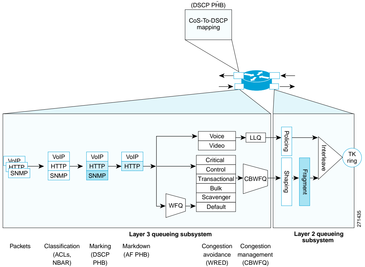
Figure 31 WAN Router
