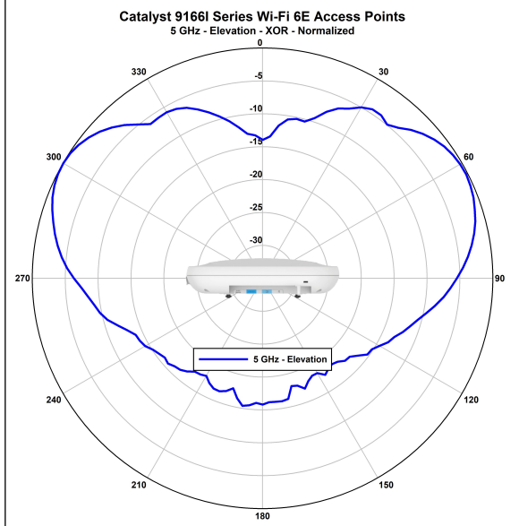
Figure 10: CW9166I - XOR Normalized Radiation Pattern (5-GHz Elevation)
