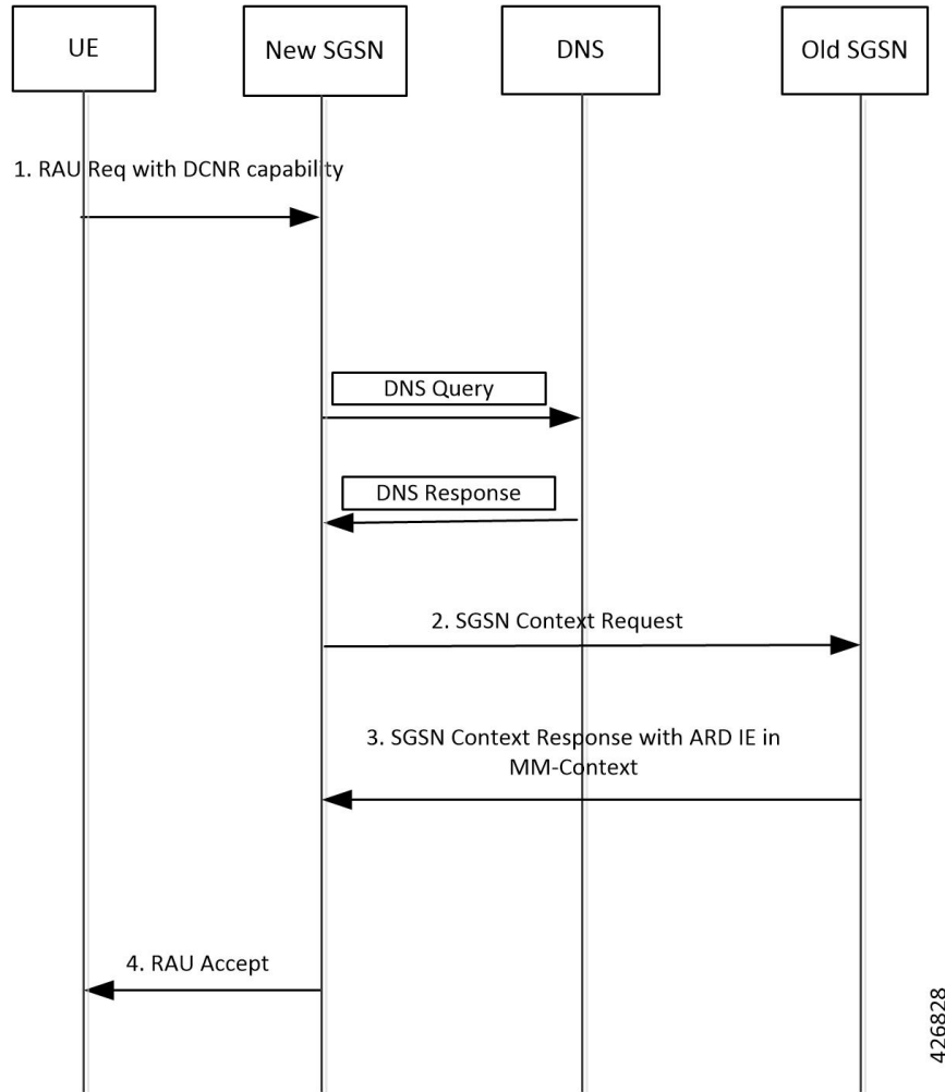
Figure 6: Inter SGSN RAU
