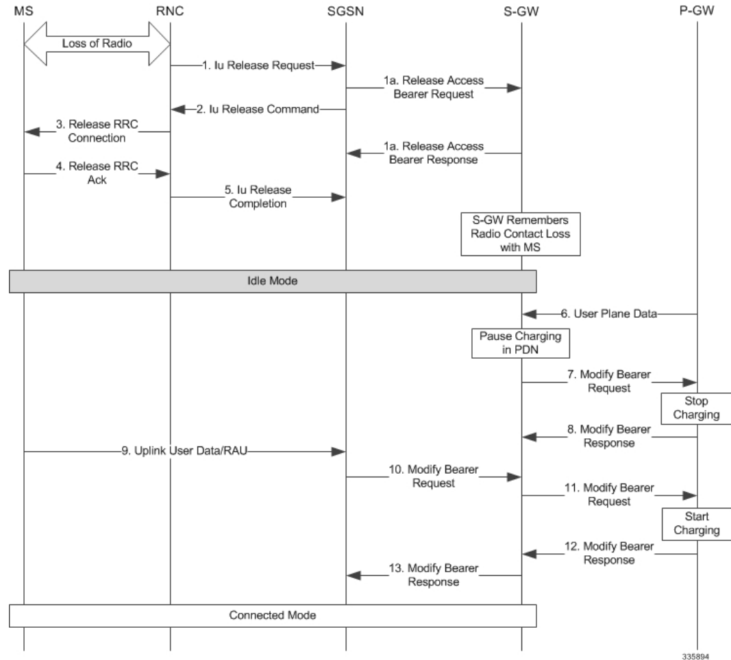
Figure 1: Iu-Release and Overcharging Protection on the S4
