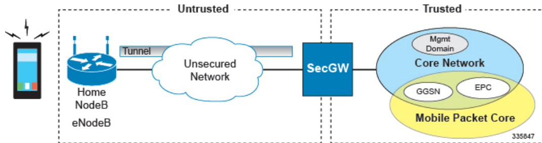
Figure 1: SecGW Implementation
