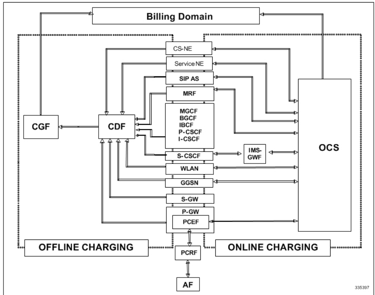
Figure 96: Charging Architecture
