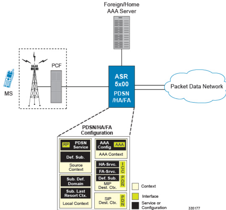
Figure 10: Simple and Mobile IP Support Within a Single System
