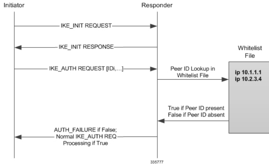
Figure 26: Whitelist Implementation
