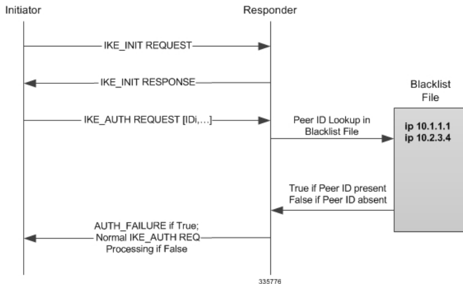
Figure 25: Blacklisting Implementation
