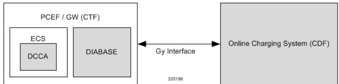
Figure 16: Gy Architecture
