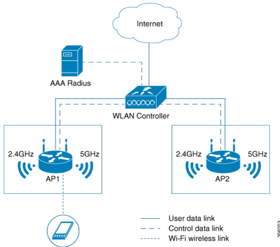
Figure 7: Wi-Fi Agile Multiband Wireless Infrastructure Network
