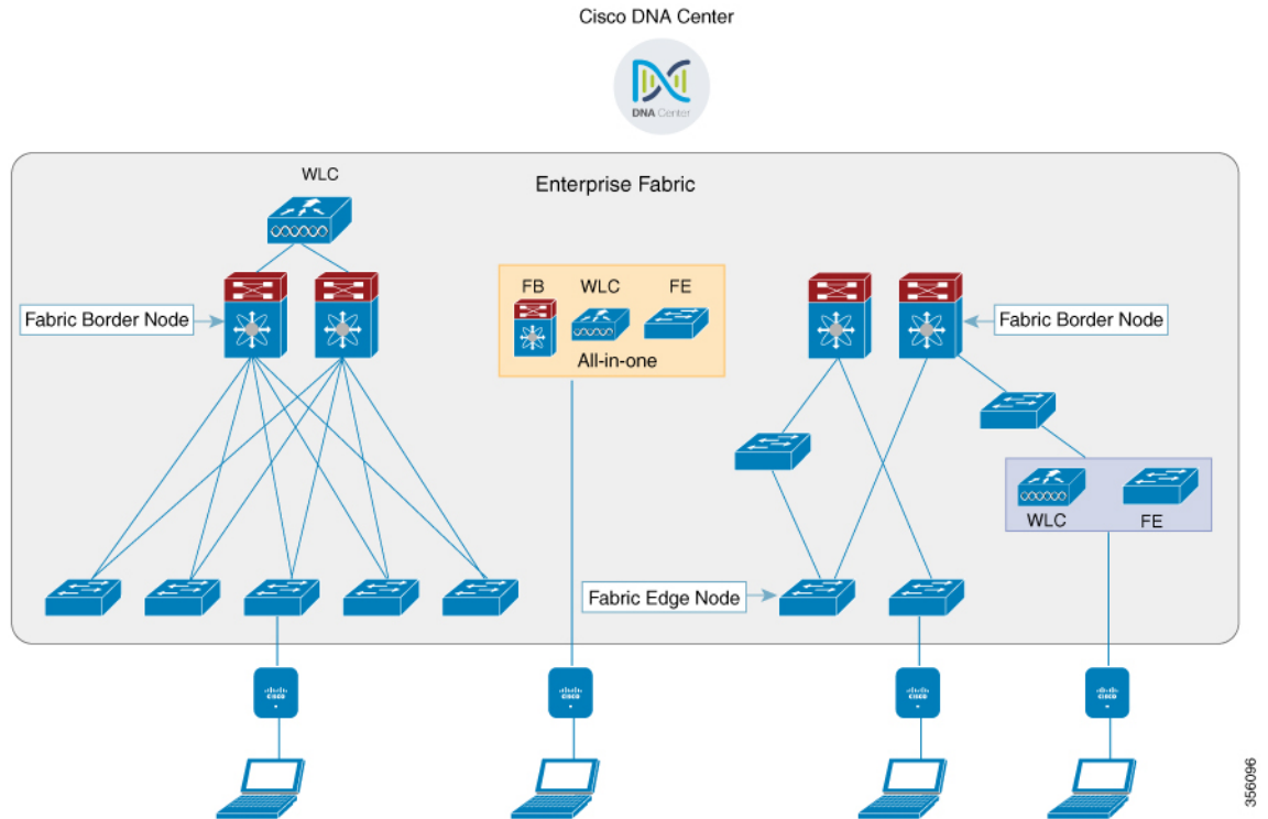
Figure 26: Software-Defined Access Wireless
