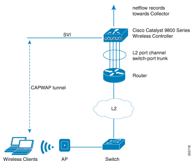
Figure 27: Encrypted Traffic Analytics Deployed on Cisco Catalyst 9800 Series Wireless Controller in Local Mode
