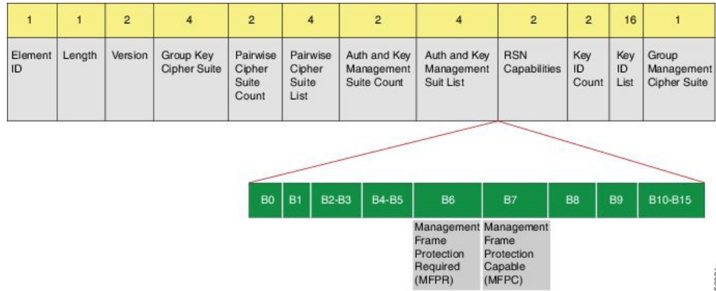
Figure 35: 802.11w Information Elements
