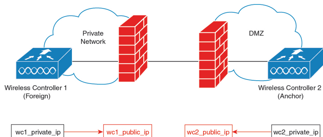
Figure 22: Mobility NAT
