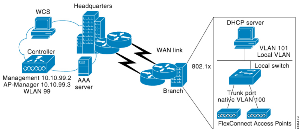
Figure 19: FlexConnect Deployment
