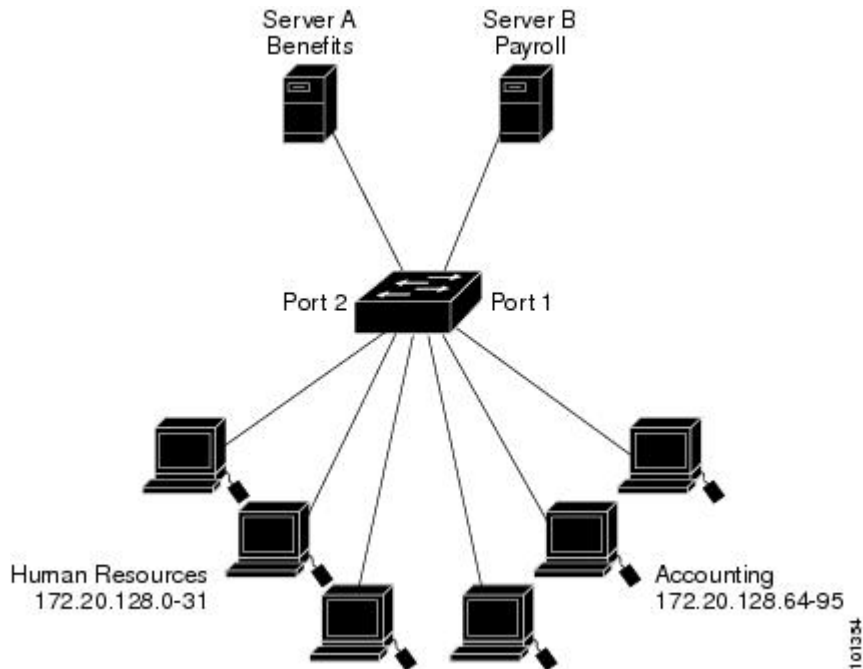
Figure 15: Using Router ACLs to Control Traffic
