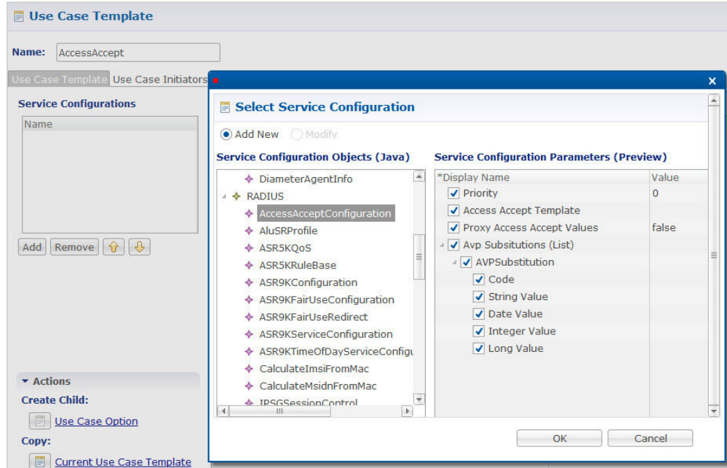
Figure 61: AccessAccept Template
