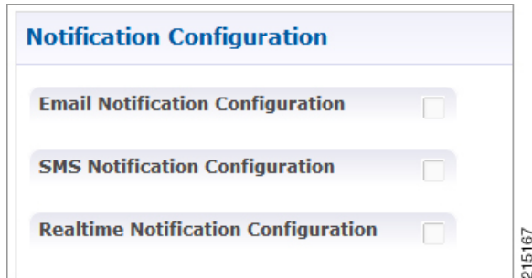
Figure 11: Notification Configuration
