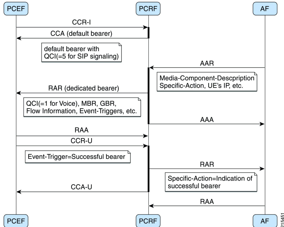
Figure 138: Example VoLTE Call
