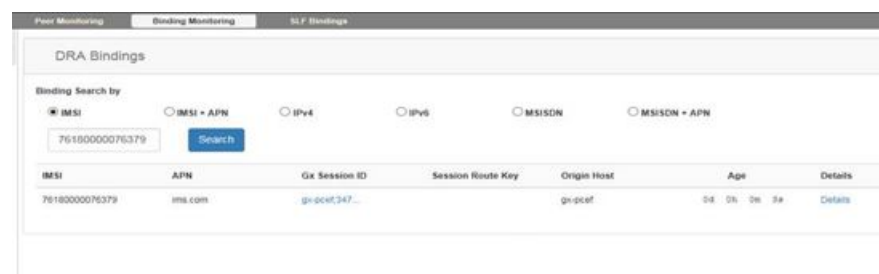
Figure 4: DRA Bindings
