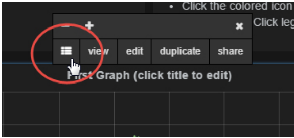
Figure 52: Rows
