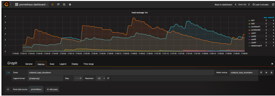
Figure 19: Sample Graph
