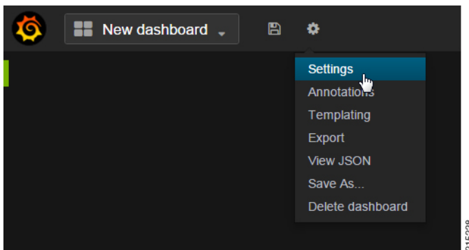
Figure 34: Settings
