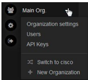
Figure 26: New Organization
