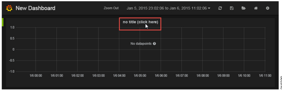
Figure 37: Edit
