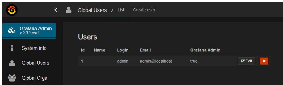
Figure 23: List Tab
