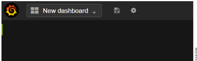
Figure 32: Blank Dashboard
