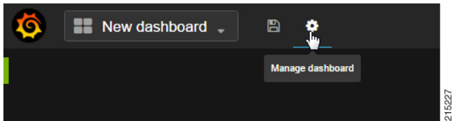
Figure 34: Settings
