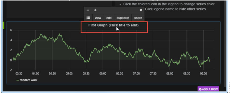
Figure 51: Title
