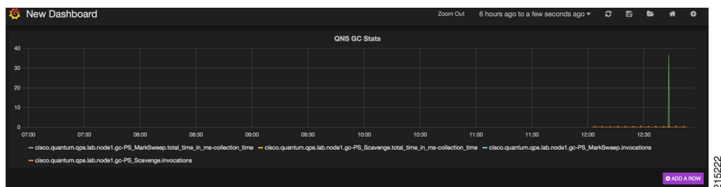
Figure 48: Example Graph
