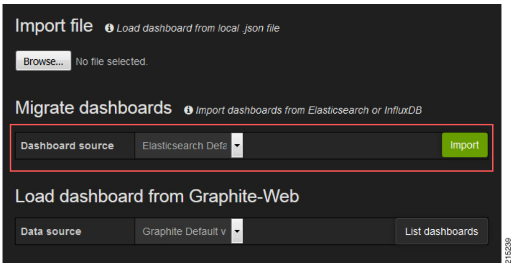
Figure 30: Import File
