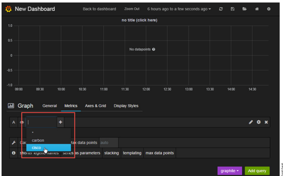
Figure 38: Metric Selection
