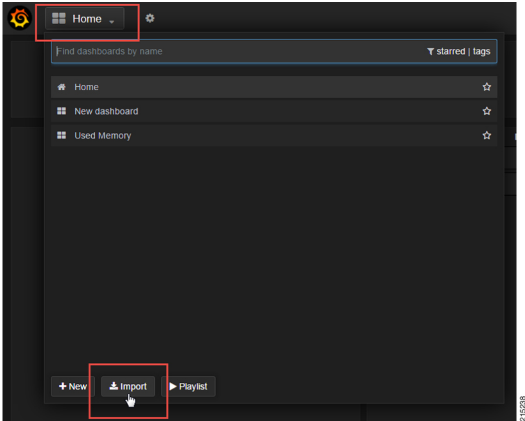
Figure 29: Import
