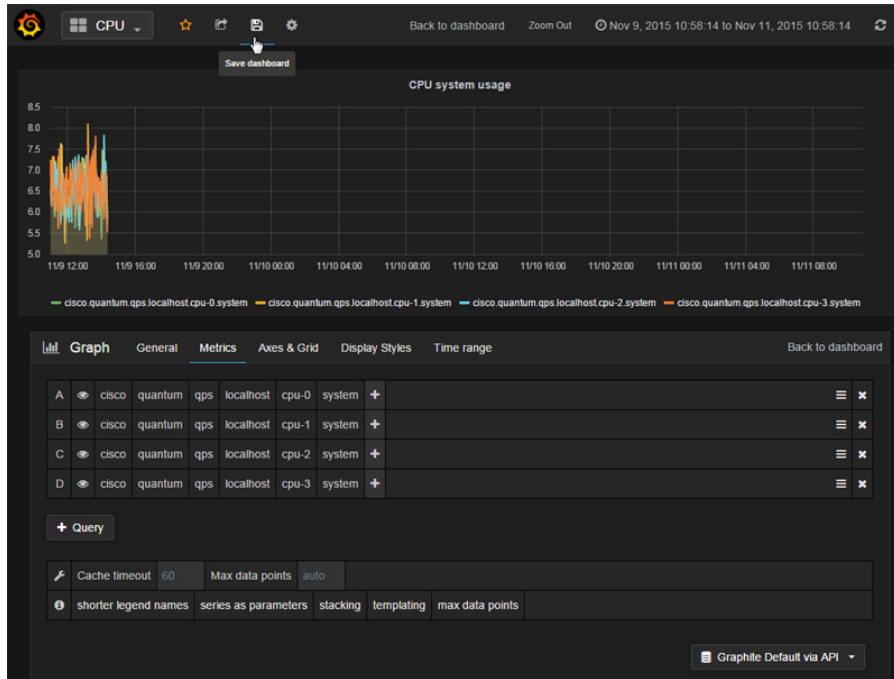
Figure 41: Save
