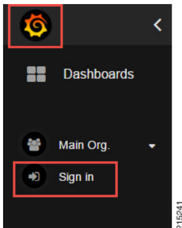
Figure 21: Grafana Logo
