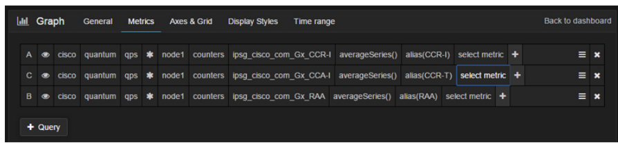
Figure 42: Graphical Representation
