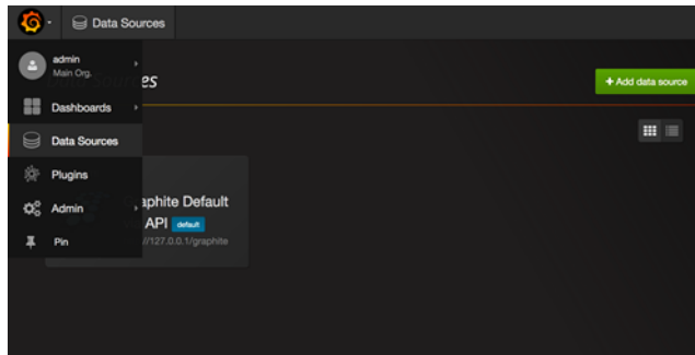
Figure 17: Sidebar Menu
