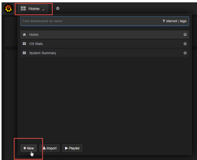
Figure 31: Home
