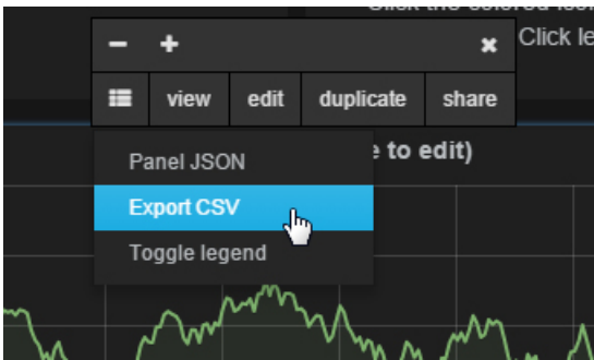
Figure 53: Export
