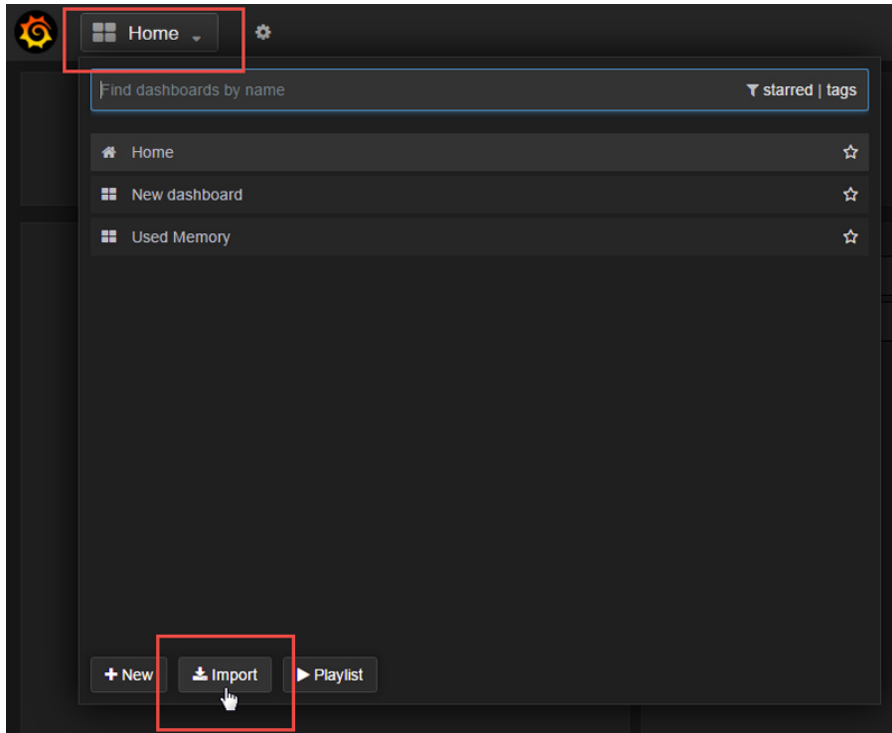
Figure 50: Import
