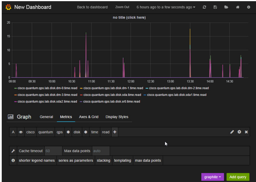
Figure 39: Aggregation Functions
