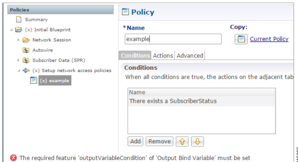
Figure 56: Error in Policy Builder
