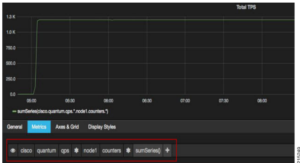
Figure 46: Total TPS
