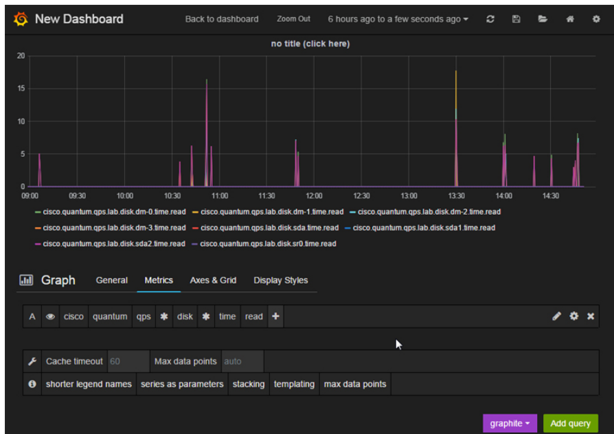
Figure 40: Aggregation Functions
