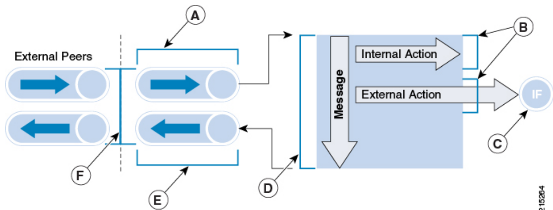
Figure 58: Various Statistic Gathering Points for Incoming and Outgoing Messages
