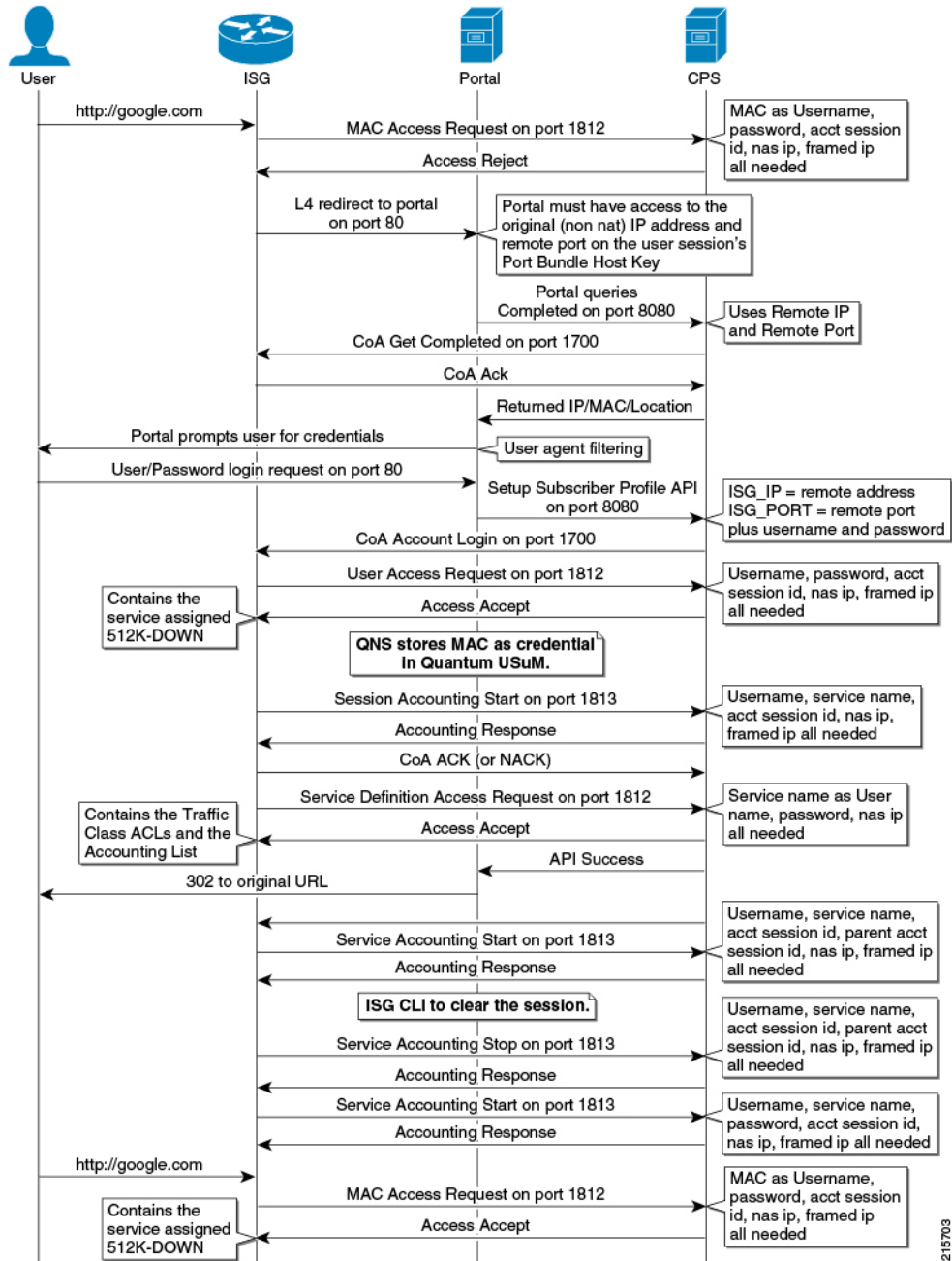
Figure 51: MAC TAL Call Flow
