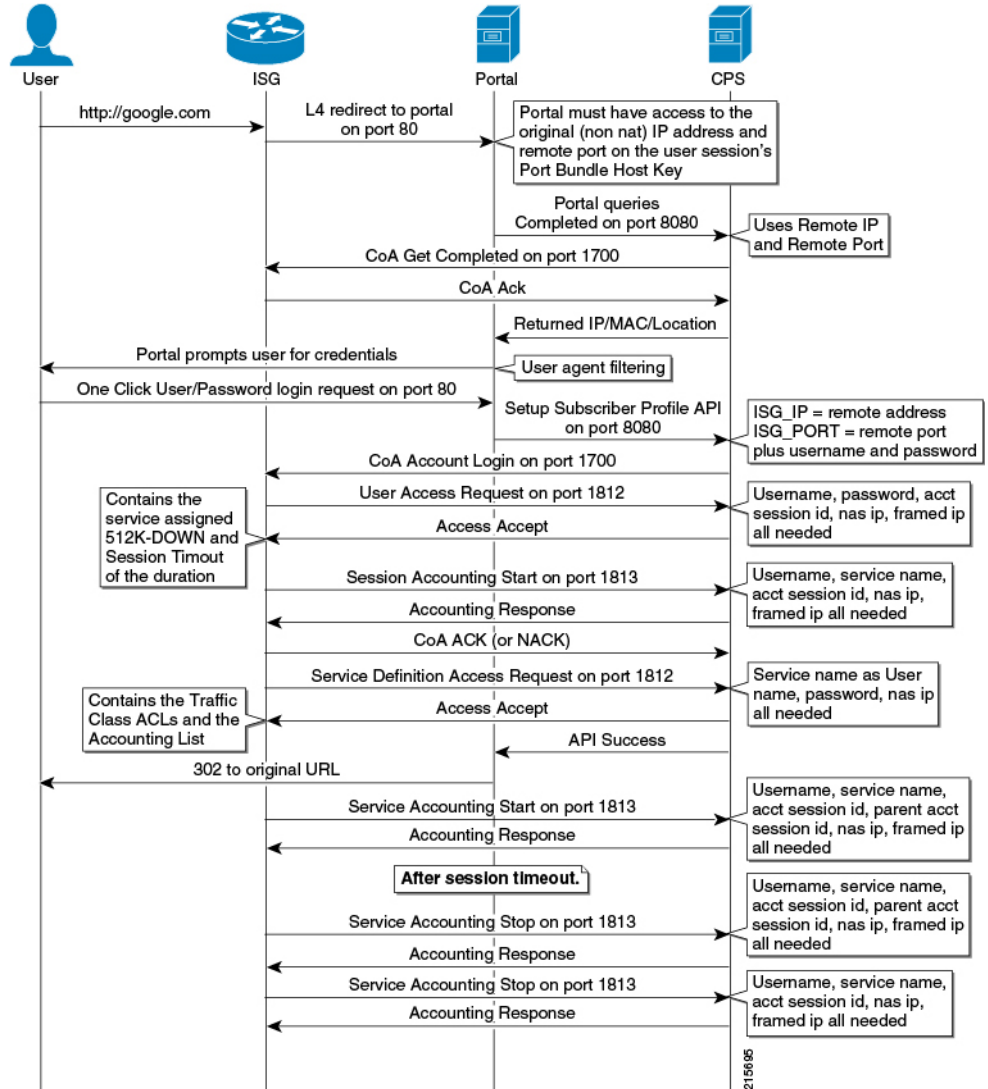
Figure 48: Time-limited Voucher Call Flow
