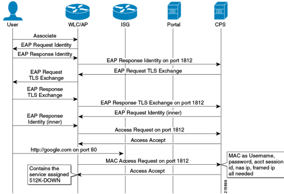
Figure 49: EAP-TTLS Call Flow
