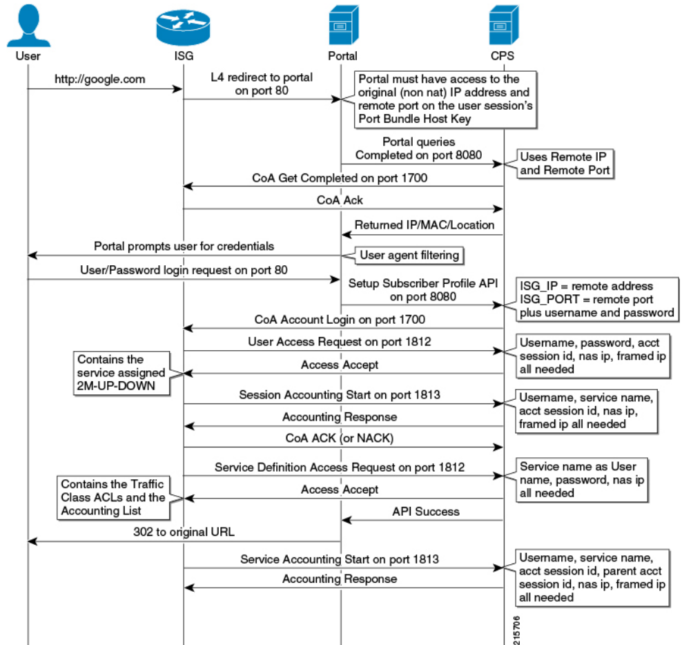
Figure 52: Tiered Services Call Flow
