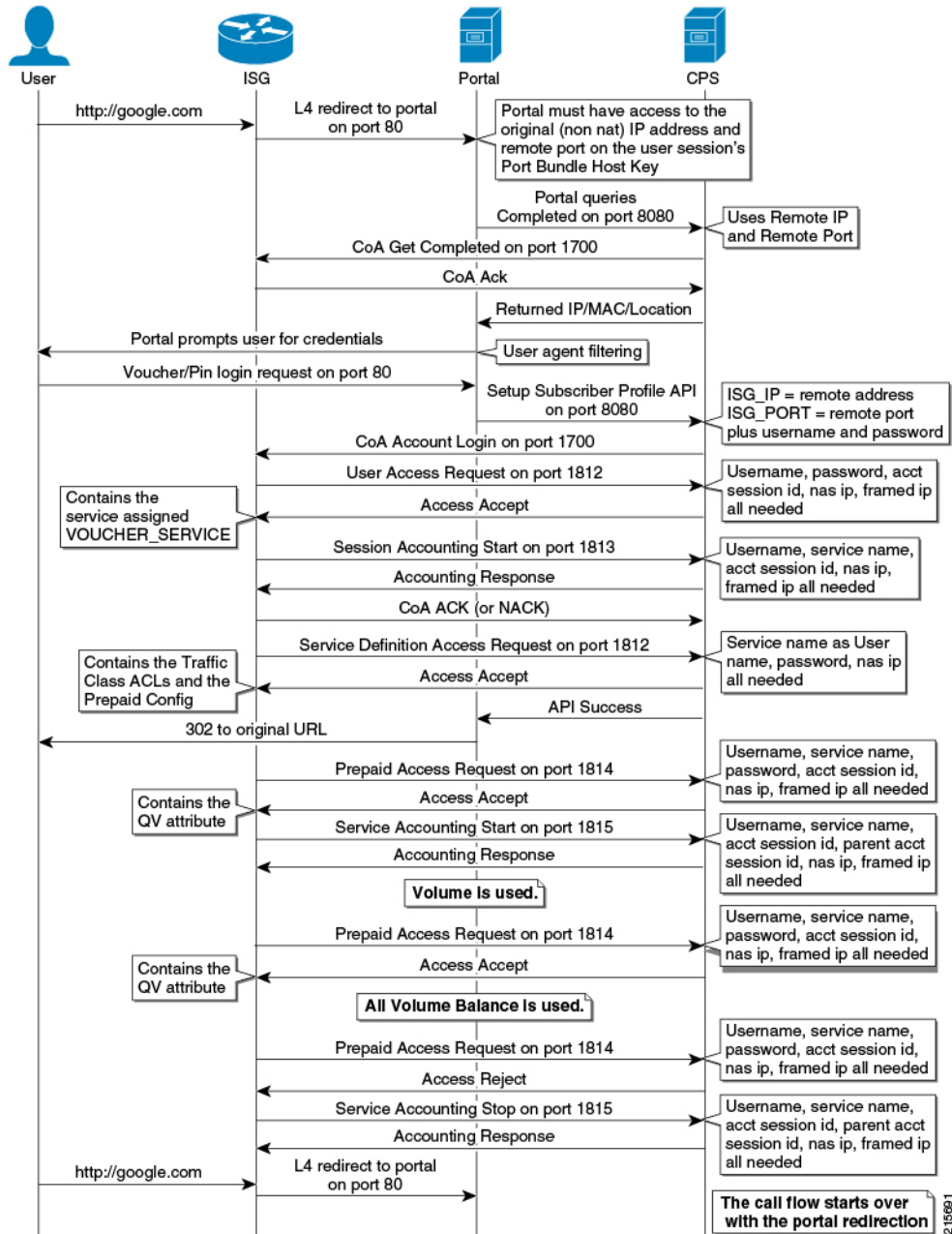
Figure 47: Data-limited Voucher Call Flow
