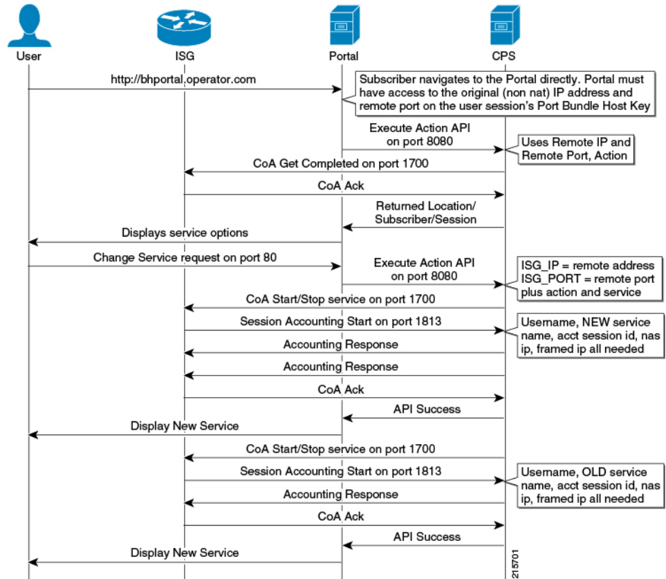
Figure 50: Service Selection Call Flow
