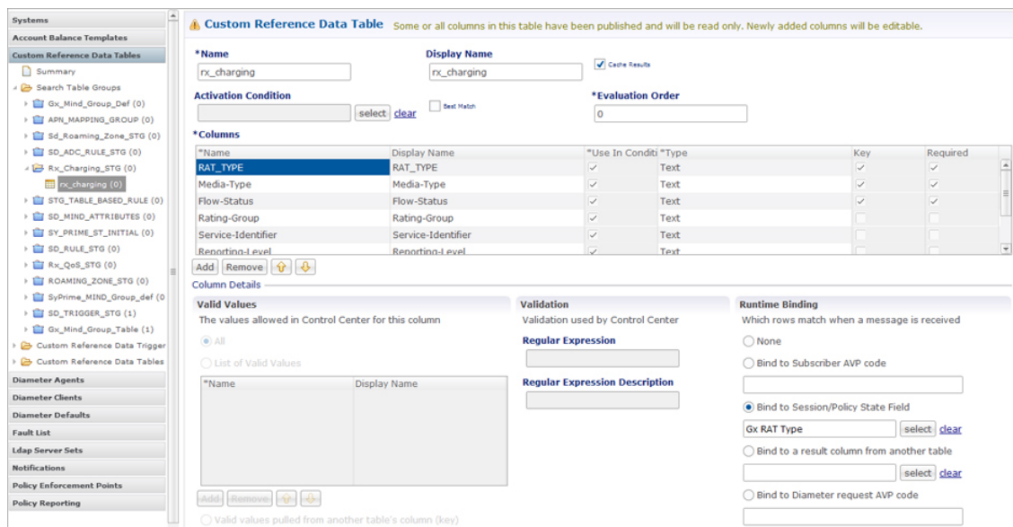
Figure 158: RAT_Type key column
