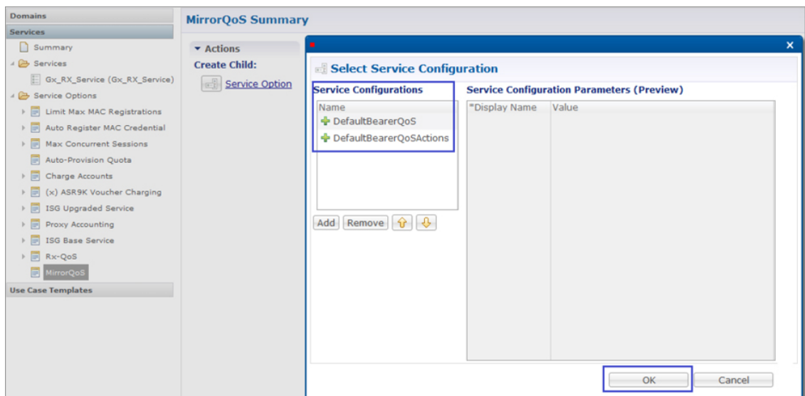
Figure 64: Mirror QoS Summary
