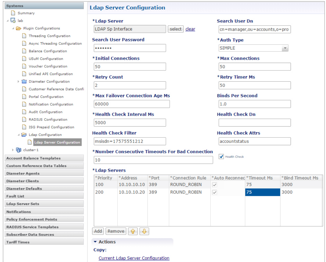
Figure 89: Ldap Server Configuration
