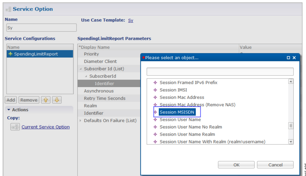
Figure 68: Session MSISDN Identifier
