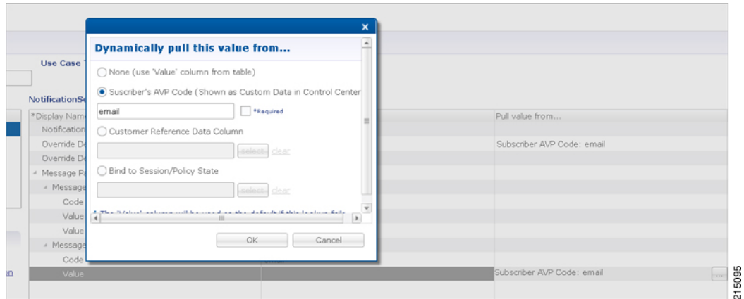
Figure 177: Subscriber AVP code Email Values
