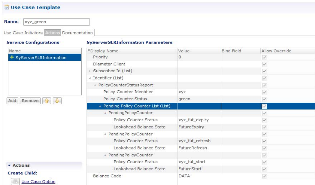
Figure 171: SyServerSLRInformation Service Configuration Object
