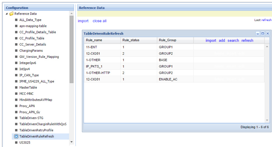
Figure 129: Configuring Reference Data
