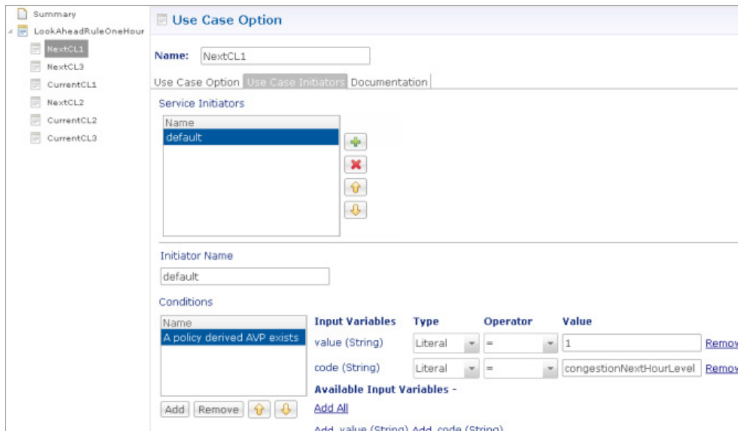
Figure 138: Use Case Initiators Tab
