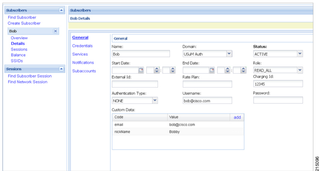
Figure 178: Subscriber General Details
