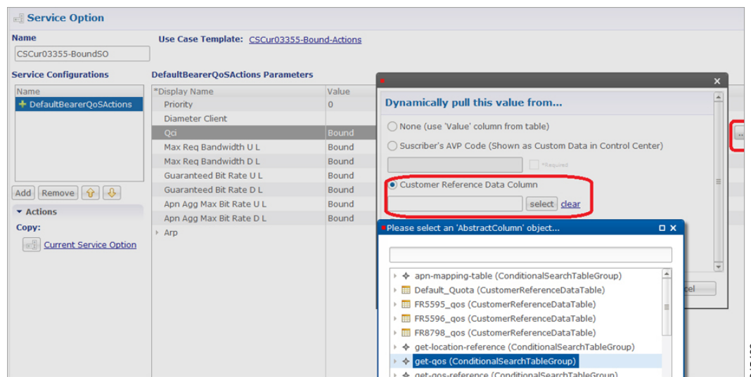
Figure 114: Custom Reference Data Column
