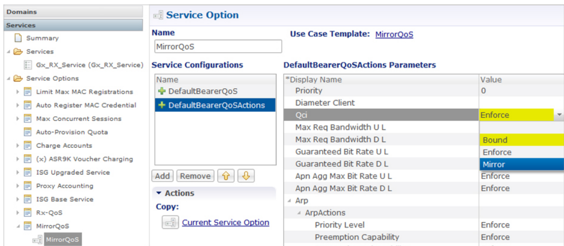
Figure 65: Mirror QoS Summary - Service Option
