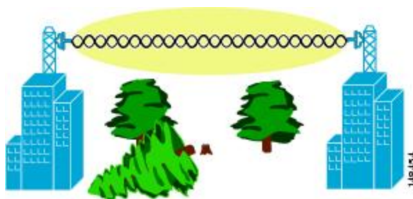
Figure 26: Removing Obstructions in a Fresnel Zone
